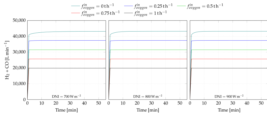
Figure 6. Syngas ( H_2 + CO ) production for various oxygen flow rates and DNI levels.
