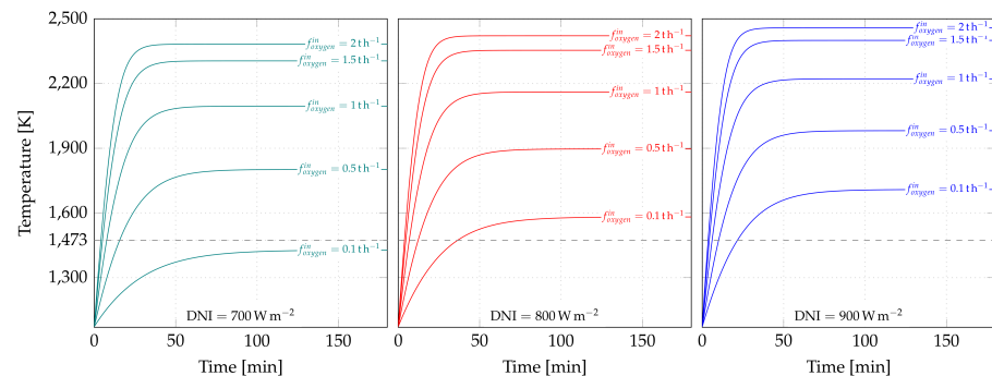
Figure 7. Evolution of the reactor's temperature for various oxygen flow rates and DNI levels ( f_{biomass}^{in} = 1.465 \text{ th}^{-1} and the initial temperature is 1073 K).
