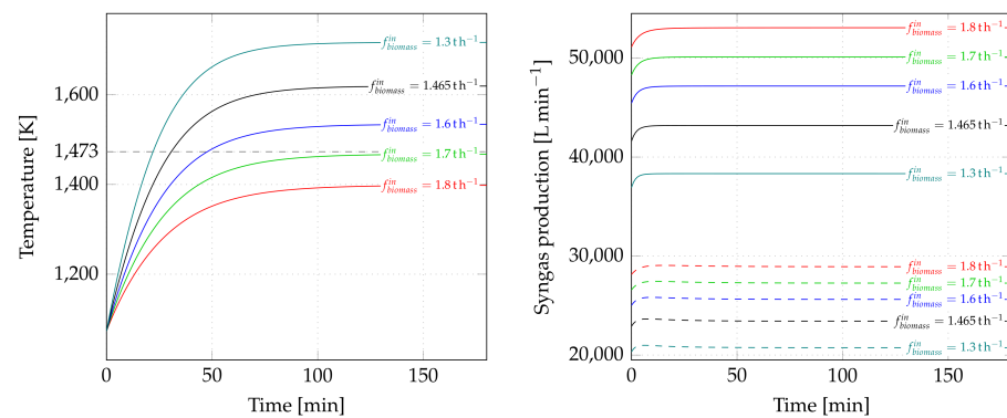
Figure 5. Evolution of the reactor's temperature for various biomass flow rates when DNI is equal to 900 \text{ W m}^{-2} and corresponding syngas production (dashed line: H_2 ; solid line: H_2 + CO ).
