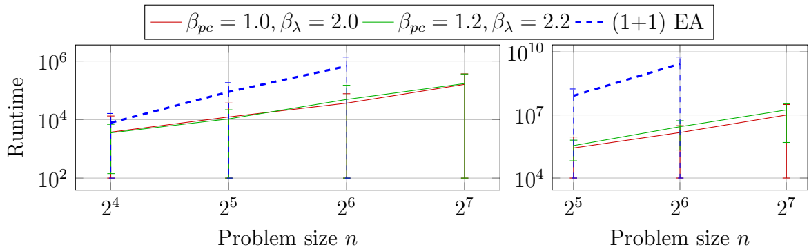
Figure 5: Running times of the heavy-tailed (1 + (\lambda, \lambda)) GA on JUMP, depending on the problem size n , in comparison to the (1 + 1) EA. Jump sizes are k = 3 on the left and k = 5 on the right.
