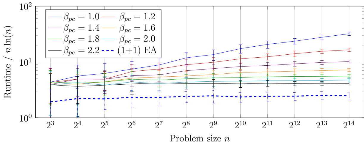
Figure 3: Running times of the heavy-tailed (1 + (\lambda, \lambda)) GA on ONEMAX starting from a random point, normalized by n \ln(n) , for different \beta_{pc} = \beta_p = \beta_c and \beta_\lambda = 2.8 in relation to the problem size n . The expected running times of (1 + 1) EA, also starting from a random point, are given for comparison.
