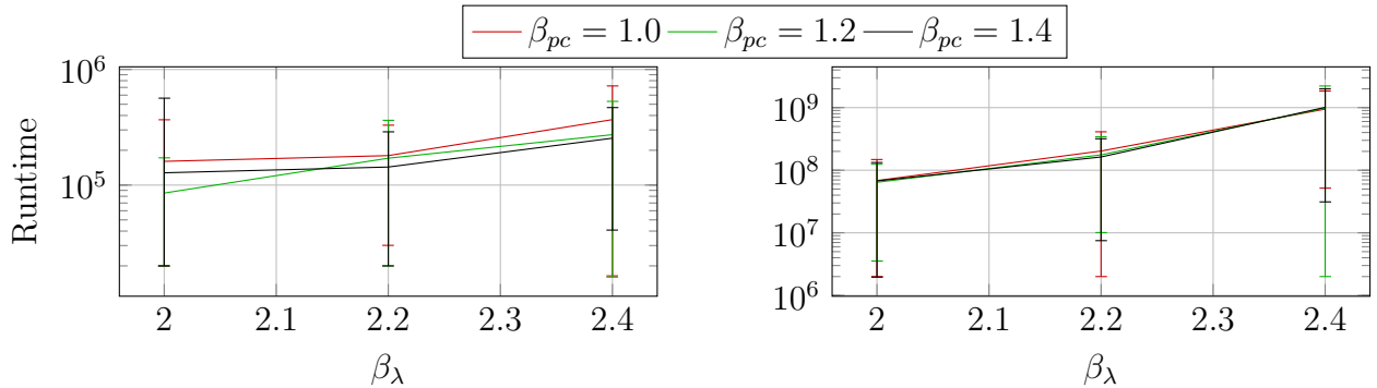
Figure 6: Dependency of running times of the heavy-tailed (1 + (\lambda, \lambda)) GA on \text{JUMP}_k on \beta_\lambda and \beta_{pc} for k = 3 (on the left) and k = 6 (on the right). Problem size n = 2^7 is used.
