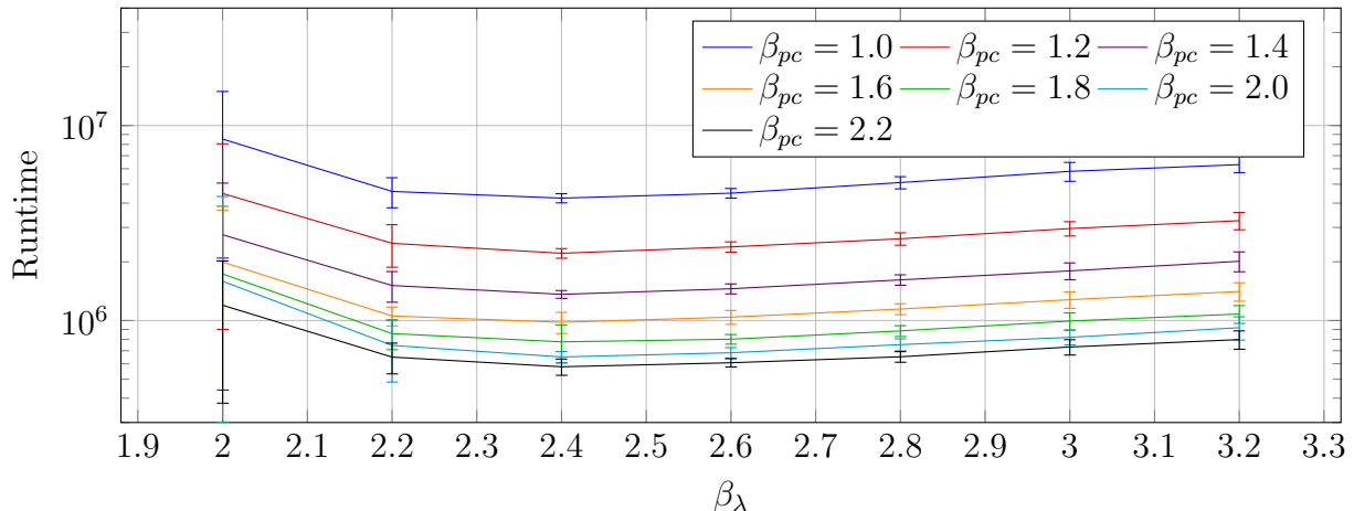
Figure 4: Running times of the heavy-tailed (1 + (\lambda, \lambda)) GA on ONEMAX starting from a random point, for n = 2^{14} and different \beta_{pc} = \beta_p = \beta_c depending on \beta_\lambda .
