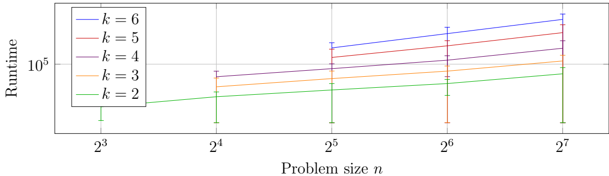
Figure 7: Running times of the heavy-tailed (1 + (\lambda, \lambda)) GA with \beta_{pc} = 1.0 and \beta_\lambda = 2.0 on \text{JUMP}_k for k \in [2..6] depending on the problem size n .
