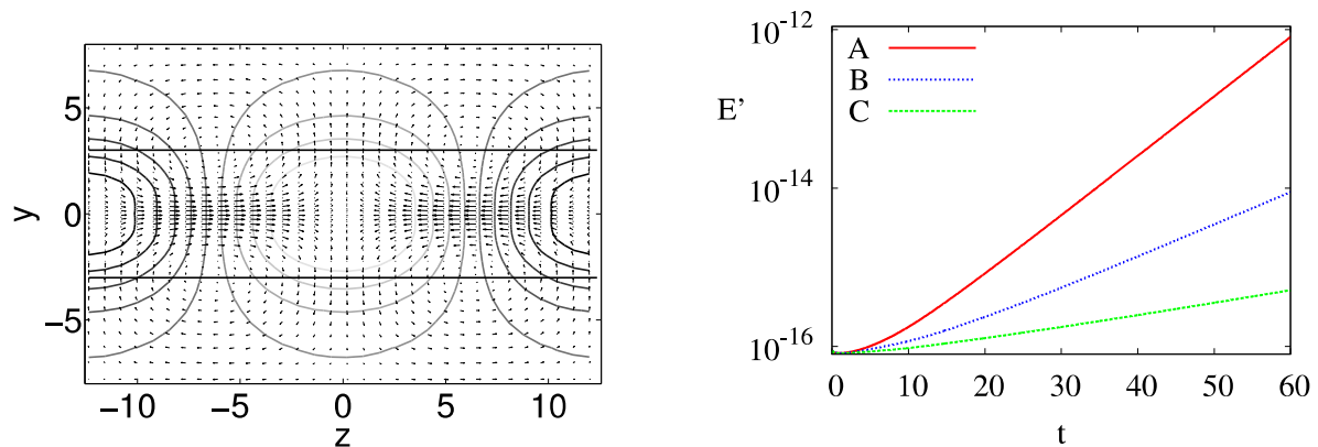
Figure 2. Left panel: Cross-stream view of the optimal initial streamwise vortices (arrows) and optimally amplified streamwise streaks (contour lines) for \beta = 0.25 . The two horizontal lines correspond to the shear layer boundary where U(y)=0.01 . The optimal initial streamwise vortices are approximately centered on this boundary and induce alternated low and high speed streaks. Right panel: Temporal evolution of the impulse response energy E' evolving on top of the 2D Bickley jet A and on the increasingly streaky jets B and C. The presence of streaks stabilizes the unstable inflectional mode.
