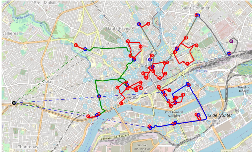
FIG. 1 – Visualization of the best found solution for instance “Nantes-50-1” with 50 customers
