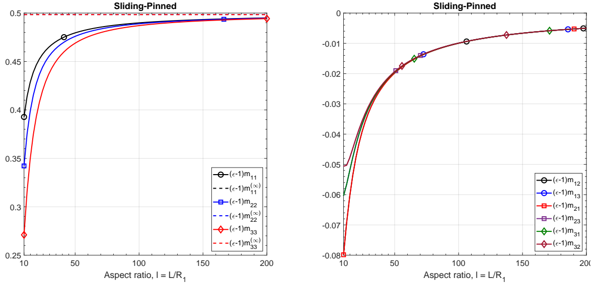
Figure E.16: Sliding-Pinned case. Evolution of the added-mass coefficient (\varepsilon - 1)m_{ij} , predicted by the equation (38), as a function of the aspect ratio l . Left : diagonal terms. The horizontal dashed lines correspond to the limit l \rightarrow \infty , given by the equation (41). Right : off-diagonal terms. These terms tend to 0 as l \rightarrow \infty . Symbols are used to distinguish superimposed curves.
