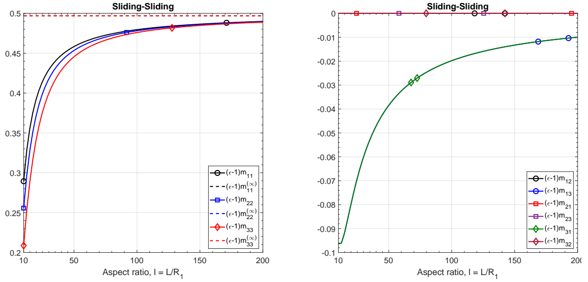
Figure E.17: Sliding-Sliding case. Evolution of the added-mass coefficient (\varepsilon - 1)m_{ij} , predicted by the equation (38), as a function of the aspect ratio l . Left : diagonal terms. The horizontal dashed lines correspond to the limit l \rightarrow \infty , given by the equation (41). Right : off-diagonal terms. These terms tend to 0 as l \rightarrow \infty . Symbols are used to distinguish superimposed curves.
