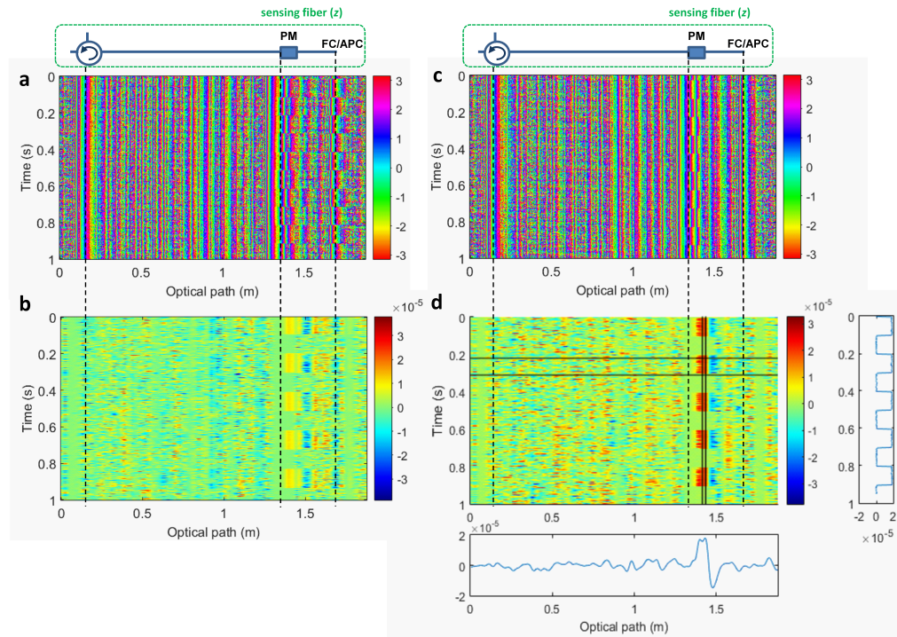
Fig. 5. a: Phase profile along the sensing fiber when a square wave signal (frequency: 5 Hz, peak-to-peak amplitude: V_{\pi}/2 ) is applied to the PM. Due to the round-trip in the sensing fiber, the phase modulation produces phase jumps of \pi between the PM and the end of the sensing fiber (i.e. for an optical path between 1.35 and 1.75 m). The color bar next to the phase plot is in radians. b: Variation of the refractive index along the fiber. An index relative variation of \approx 1.0 \times 10^{-5} is measured over a 6 cm-long optical path region that corresponds to the active area of the PM. c: The amplitude of the voltage applied to the PM is now V_{\pi} . Due to the round-trip, the modulation of the accumulated phase vanishes between the PM and the end of the sensing fiber. d: The index variation measured in the active region of the PM is \approx 1.9 \times 10^{-5} , i.e. close to twice to that of a and b. The two insets show the profiles of the index variations along the vertical and the horizontal stripes.
