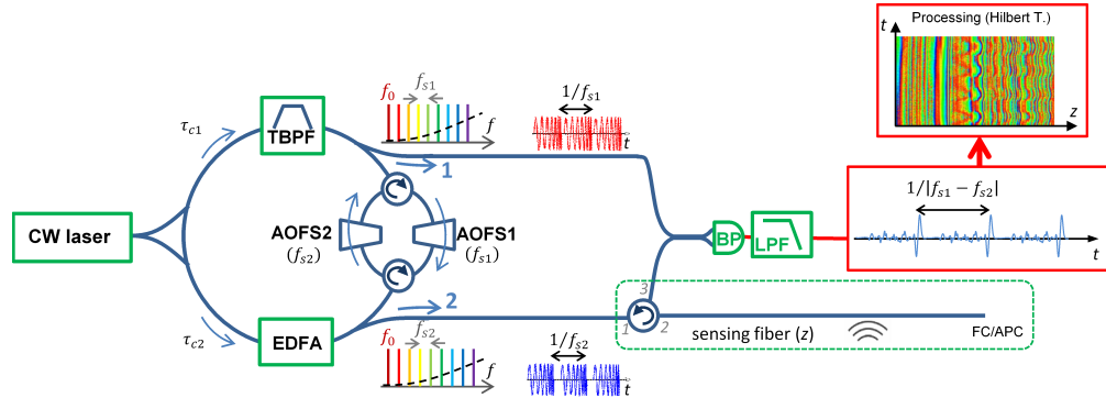
Fig. 1. Sketch of the experimental set-up. The Bi-FSL seeded with a CW laser (freq: f_0 ) generates two counter-propagating and mutually coherent optical frequency combs with slightly different frequency spacings ( f_{s1} and f_{s2} ), but identical quadratic spectral phases (see text). The corresponding waveforms in the time domain consist of trains of identical chirps, with slightly different repetition rates. After probing the sensing fiber, path #2 is recombined with the reference (path #1) on a balanced photo-detector (BP). After low-pass filtering (LPF), the signal trace (resulting from pulse compression) reproduces periodically (period: 1/\Delta f ) the real part of the reflectivity profile integrated over the fiber. Digital processing involving Hilbert transform enables to reconstruct the modulus and phase profiles along the sensing fiber.
