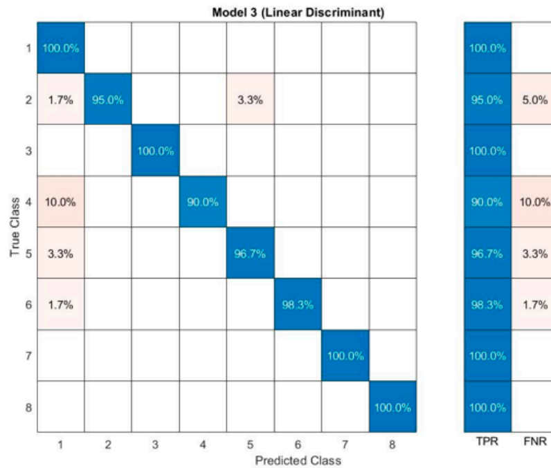
Figure 9. Linear-discriminant-model confusion matrices.
