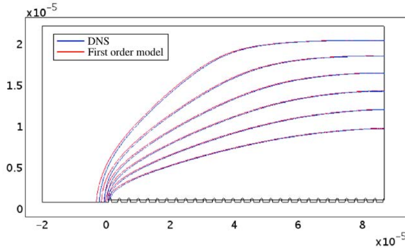
Figure 2: Concentration field contours for the initial and the effective domain, for a flow entrance velocity of 1\text{m}\cdot\text{s}^{-1} and Schmidt number of 1.
