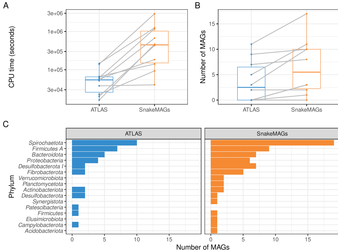
Figure 2. Comparison of the performance of SnakeMAGs v1.1.0 with another workflow, namely ATLAS v2.9.14 using 10 termite gut metagenomes. A. CPU time (in seconds) required to process each metagenome. B. Number of MAGs reconstructed from each metagenome. On both boxplots, gray lines link the result obtained with ATLAS and the one obtained with SnakeMAGs for each of the 10 analyzed termite metagenomes. C. Number of bacterial MAGs at the phylum level recovered from each workflow.
