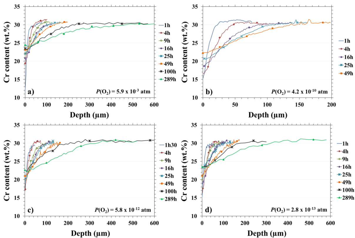
Figure 3: Chromium depletion profiles in Ni-30Cr alloy after oxidations at 1150 °C a) in 5.9 \times 10^{-3} atm O_2 ; b) in 4.2 \times 10^{-10} atm O_2 ; c) 5.8 \times 10^{-12} atm O_2 ; d) 2.8 \times 10^{-13} atm O_2 .
