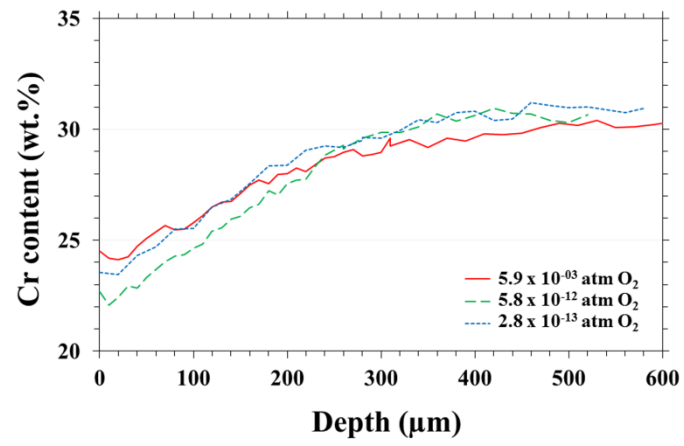
Figure 4: Chromium depletion profiles in Ni-30Cr after oxidations of 100h in different oxygen partial pressures at 1150 °C.
