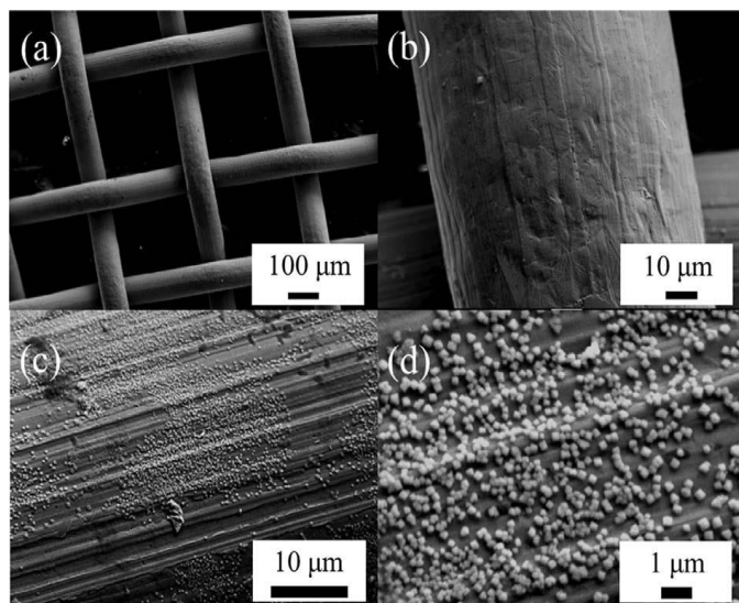
Fig.6. SEM characterization of the stainless-steel cathode (a) and (b) Pristine stainless-steel mesh. (c) and (d) Coated stainless steel mesh with copper deposits after the electrode sorption experiments.
