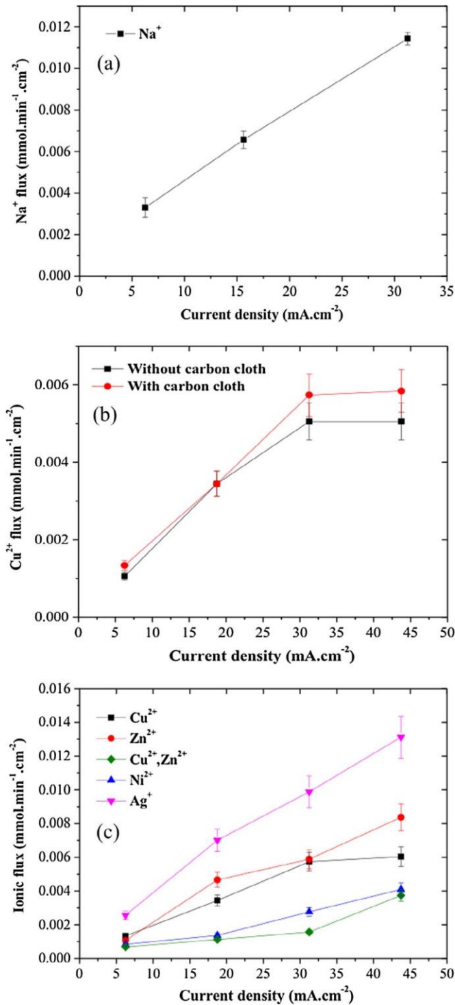
Fig.2. Ionic fluxes across the ED microfluidic device from the diluate to the concentrate compartment as a function of the current density. (a) Sodium ( \text{Na}^+ ) ionic fluxes without carbon cloth. (b) Copper ( \text{Cu}^{2+} ) ions fluxes with and without carbon cloth. (c) Ionic fluxes with carbon cloth for the different heavy metal ions studied.
