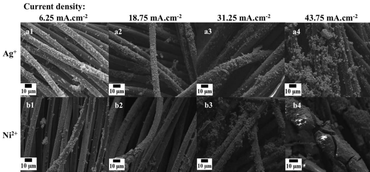
Fig. 4. SEM characterization of the metal deposits. (a) Silver and (b) nickel deposits on the carbon cloth as a function of the current densities at 6.25 (1), 18.75 (2), 31.25 (3) and 43.75 (4) mA • cm -2 .
