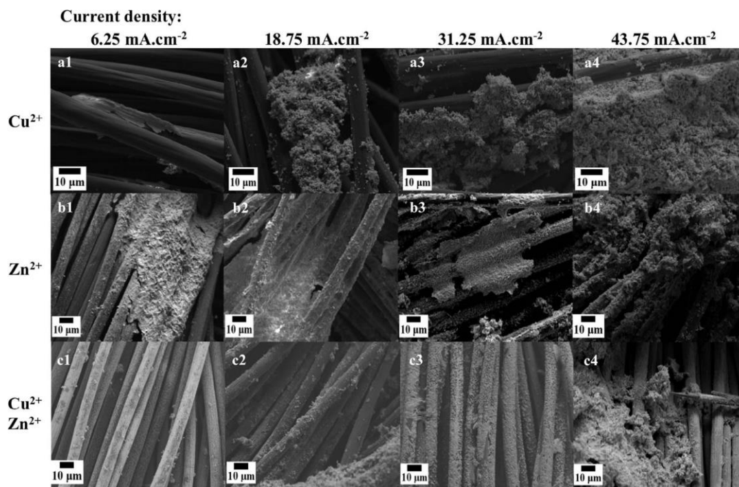
Fig. 3. SEM characterization of the metal deposits. (a) Copper, (b) zinc and (c) mixed copper/zinc deposits on the carbon cloth as a function of the current densities at 6.25 (1), 18.75 (2), 31.25 (3) and 43.75 (4) \text{mA} \cdot \text{cm}^{-2} .
