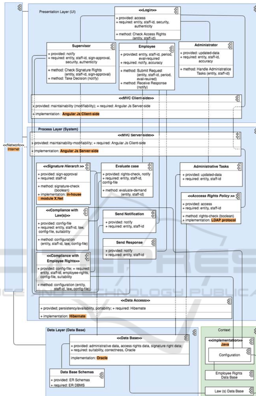
Figure 1: The VRS RA of the S-SEDT HR system with components' interfaces; in orange the variants' choices.
