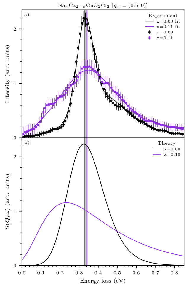
FIG. 5. Comparison between experiment and theory at \mathbf{q}_{\parallel} = (0.5, 0) for \text{Na}_x\text{Ca}_{2-x}\text{CuO}_2\text{Cl}_2 . (a) Cu L_3 -edge RIXS data for x = 0.00 at \mathbf{q}_{\parallel} = (0.49, 0) (black circle) and x = 0.11 at \mathbf{q}_{\parallel} = (0.51, 0) (purple square). The fits are shown as solid lines in black ( x = 0.00 ) and purple ( x = 0.11 ). The background, phonon, and elastic contributions have been subtracted from both the data and fits to compare with theory. The energy of the fitted magnon (paramagnon) at x = 0.00 ( x = 0.11 ) is shown as a vertical black (purple) line. (b) CDMFT calculations at x = 0.00 (black) and x = 0.1 (purple). The calculated spectra have been multiplied by a Bose factor with experimental temperature (22 K) and convolved with the experimental resolution function (83 meV FWHM).
