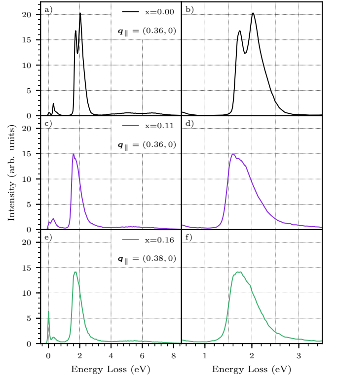
FIG. 2. Cu L_3 -edge RIXS spectra measured around the in-plane projected wavevector \mathbf{q}_{\parallel} = (0.37, 0) for x = 0.00 (a,b), x = 0.11 (c,d), and x = 0.16 (e,f) \text{Na}_x\text{Ca}_{2-x}\text{CuO}_2\text{Cl}_2 samples. The left column (a,c,e) shows the full energy domain with the quasielastic lines and phonons at lower energy, the magnetic excitations around 0.2–0.4 eV, the dd excitations around 1–3 eV, and the charge-transfer excitations around 4–8 eV. The right column (b,d,f) displays a zoom on the dd excitations to highlight their evolution with doping.
