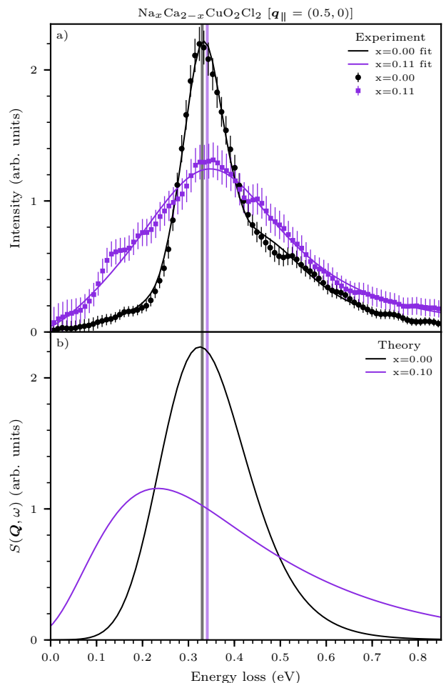
FIG. 5. Comparison between experiment and theory at q_{\parallel} = (0.5, 0) for \text{Na}_x\text{Ca}_{2-x}\text{CuO}_2\text{Cl}_2 . (a) Cu L_3 -edge RIXS data for x = 0.00 at q_{\parallel} = (0.49, 0) (black circle) and x = 0.11 at q_{\parallel} = (0.51, 0) (purple square). The fits are shown as solid lines in black ( x = 0.00 ) and purple ( x = 0.11 ). The background, phonon, and elastic contributions have been subtracted from both the data and fits to compare with theory. The energy of the fitted magnon (paramagnon) at x = 0.00 ( x = 0.11 ) is shown as a vertical black (purple) line. (b) CDMFT calculations at x = 0.00 (black) and x = 0.1 (purple). The calculated spectra have been multiplied by a Bose factor with experimental temperature (22 K) and convolved with the experimental resolution function (83 meV FWHM).
