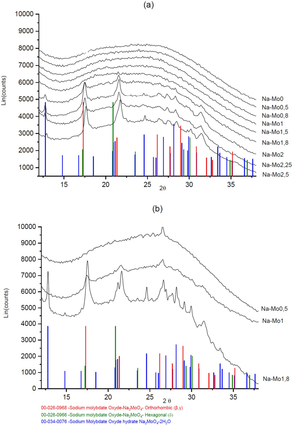
Figure 4: XRD patterns of the quenched (a) and annealed (b) Na-Mox glasses.
