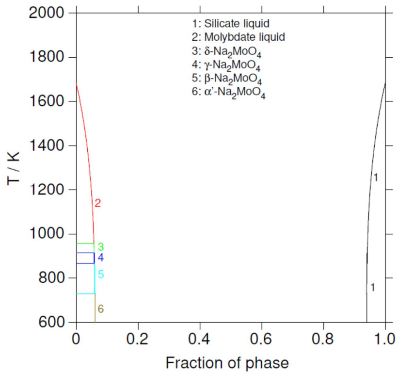
Figure 11. Calculated metastable solidification path of a \text{MoO}_3\text{-Na}_2\text{O-SiO}_2 ternary glass having a ratio \text{SiO}_2/\text{Na}_2\text{O} \approx 4 and containing 3 mol.% \text{MoO}_3 .
