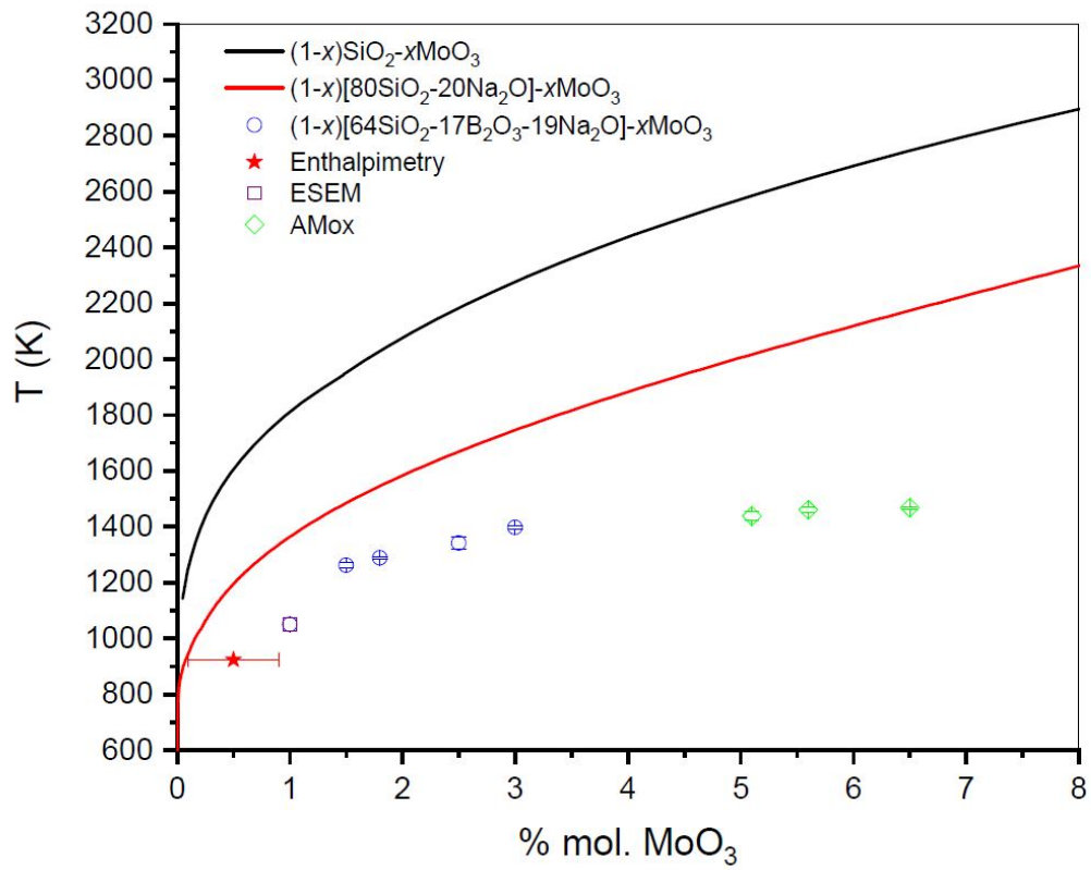
Figure 12: Phase separation temperatures calculated as a function of the MoO 3 content for SiO 2 -MoO 3 binary (black solid line) and SiO 2 -Na 2 O-MoO 3 ternary (red solid line) compositions. Comparison with the phase separation temperatures measured in this work for the SiO 2 -Na 2 O-B 2 O 3 -MoO 3 quaternary glasses and in previous study on complex AMox glass compositions (9).
