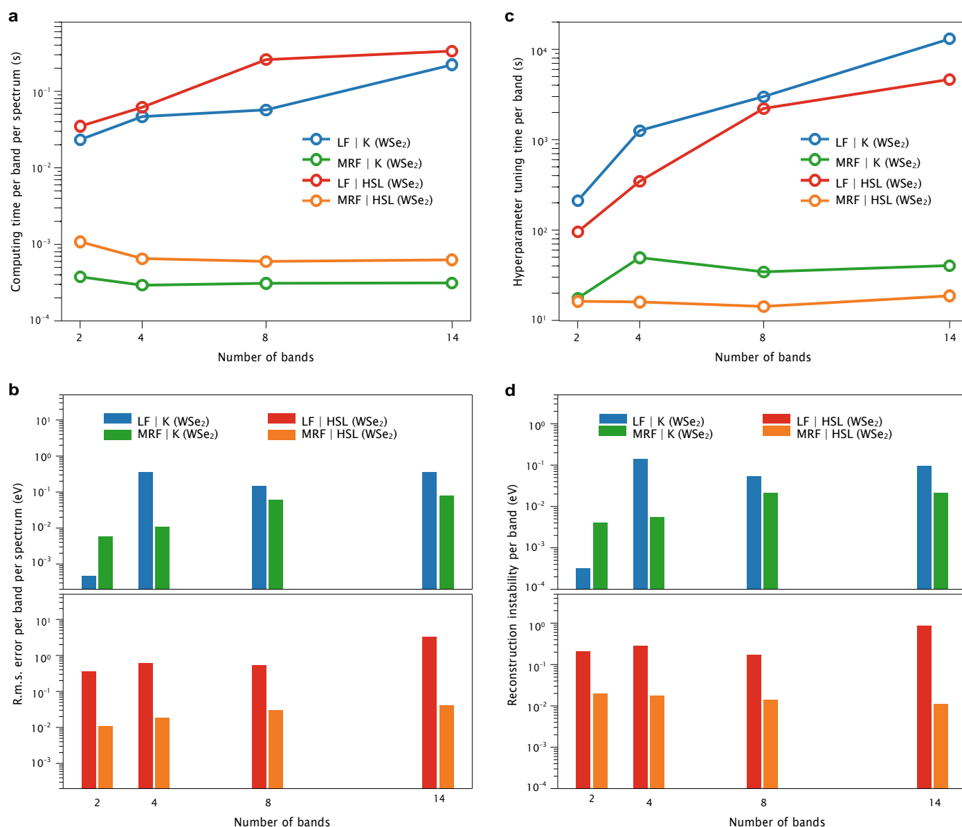
Fig. 4 | Performance evaluation on benchmarks. Visual summary of the benchmarking outcomes for BS reconstruction using normalized metrics that are able to compare across datasets. a, b , Computing time ( a ) and same-resolution r.m.s. error (reconstruction error) ( b ), both normalized to the per-band, per-spectrum level 40 . c, d , Hyperparameter tuning time ( c ) and reconstruction instability (s.d. of the residuals) ( d ), normalized to the per-band
