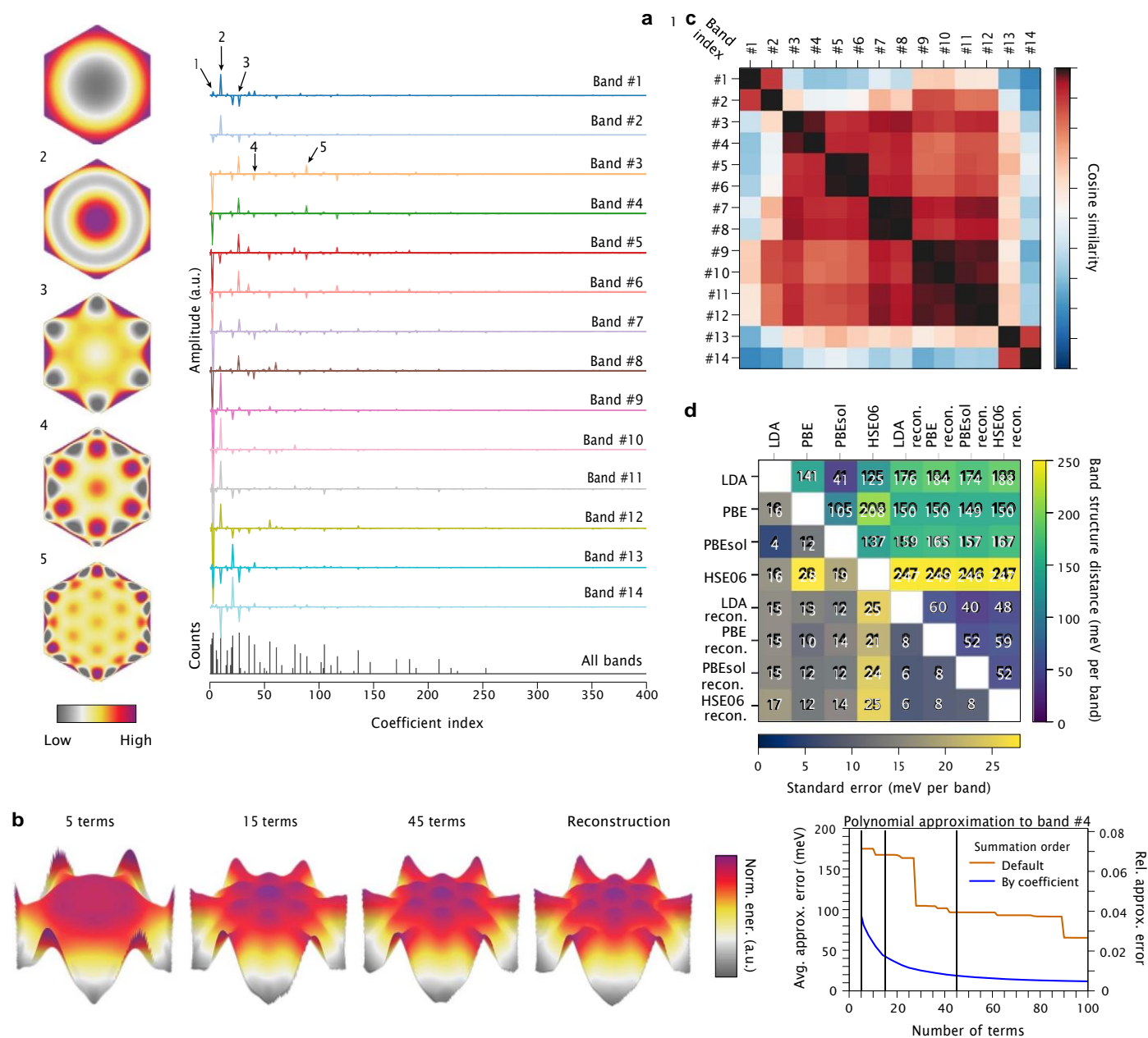
Fig. 3 | Digitization and comparison of WSe 2 BSs. a , Decomposition of the 14 energy bands of WSe 2 into hexagonal ZPs, with selected major terms displayed on the left. The zero spatial frequency term in the decomposition is subtracted for each band. The counts of large ( >10^{-2} by absolute value) coefficients of all 14 bands are accumulated in the bottom row of the decomposition to illustrate their distribution; these decrease towards higher-order terms. b , Approximation of the shape (or dispersion) of the fourth energy band using 5, 15 and 45 hexagonal ZPs are compared with the reconstruction. The three approximated ones are
