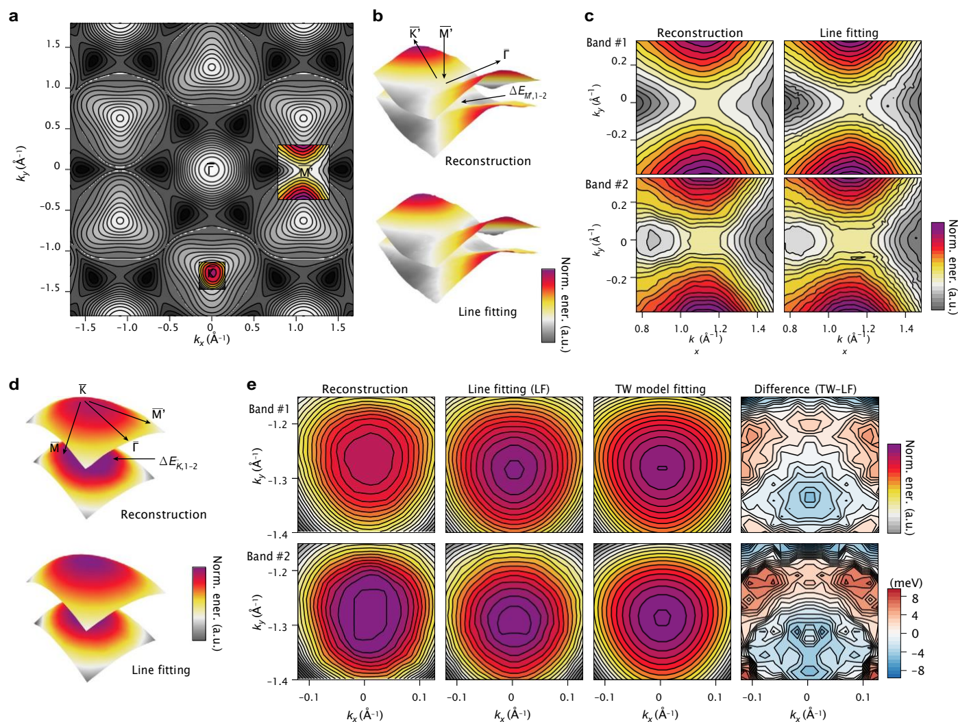
Fig. 5 | Local BS parameters of WSe 2 . a , The first valence band of 2H-WSe 2 , with constant-energy contours, from LDA-DFT calculation. The patches overlaid in color around high-symmetry points \bar{K} and \bar{M} are from reconstruction (with LDA-DFT as the initialization). b, c , Patch around the \bar{M} -point, a saddle point in the dispersion surface, visualized in 3D ( b ) and 2D ( c ). The energy gap at \bar{M} due
