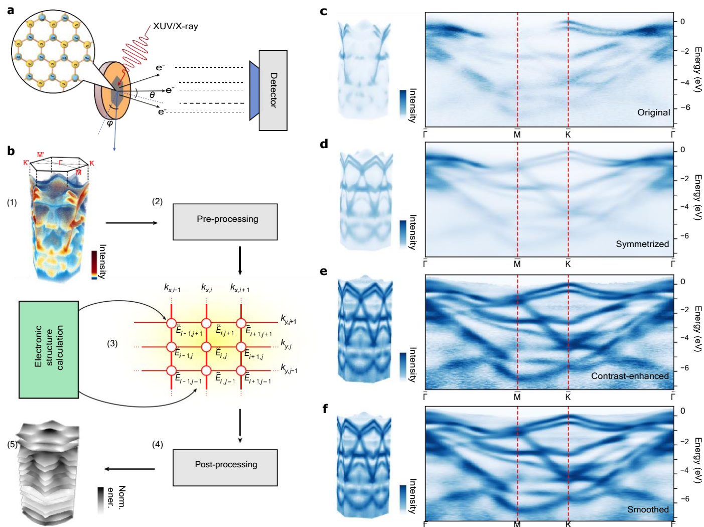
Fig. 1 | From band mapping to BS. a , Schematic of a photoemission band-mapping experiment. The electrons from a crystalline sample's surface are liberated by extreme-ultraviolet (XUV) or X-ray pulses and collected by a detector through either angular scanning or time-of-flight detection schemes. b , Overview of the computational framework for reconstruction of the photoemission (or quasiparticle) BS: (1) the volumetric data obtained from a band-mapping experiment (2) go through pre-processing steps, then are (3) fed into the probabilistic machine-learning algorithm along with electronic structure calculations as initialization of the optimization. The reconstruction algorithm for volumetric band-mapping data is represented as a 2D probabilistic
