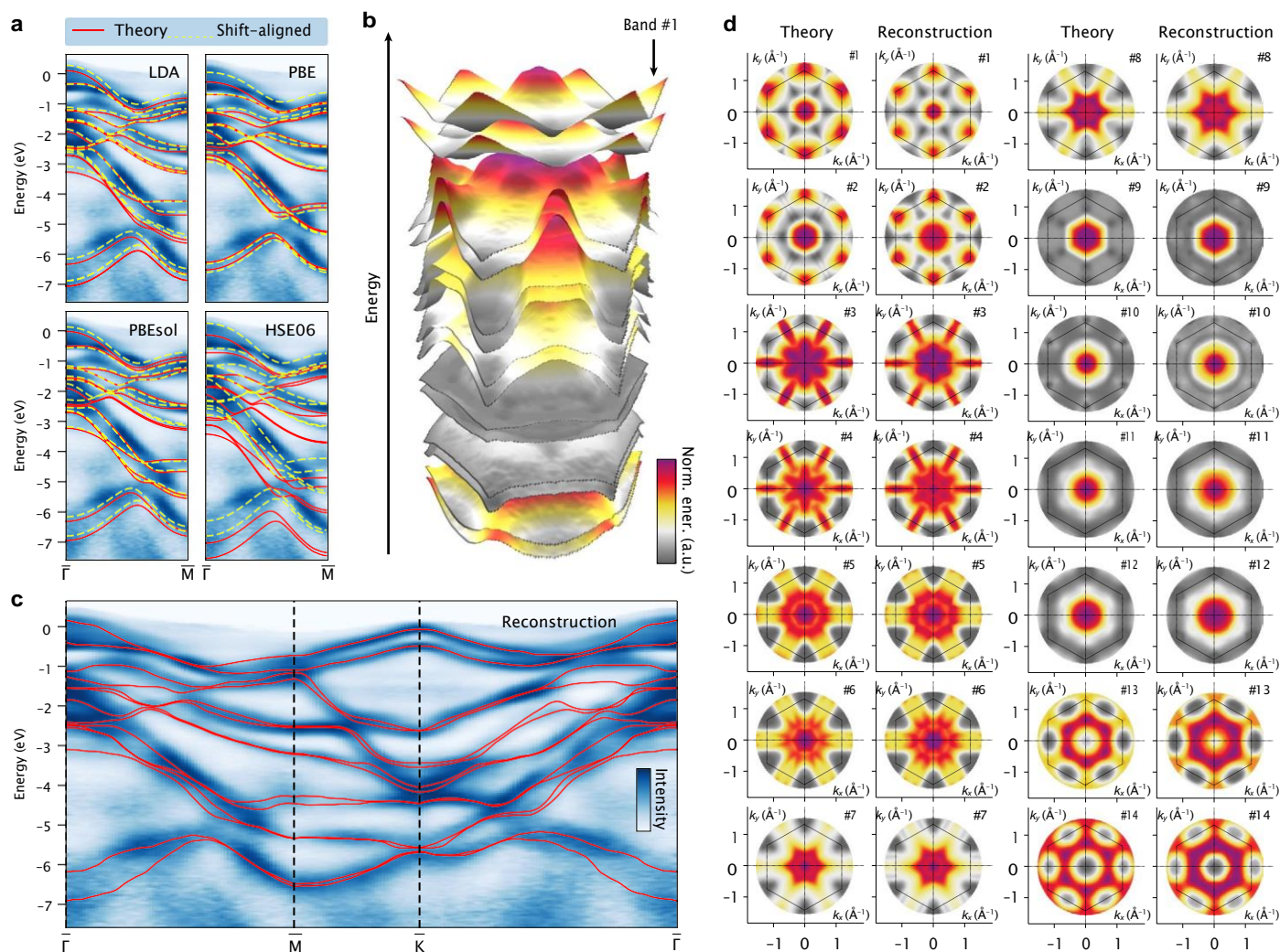
Fig. 2 | Band reconstruction from WSe 2 photoemission data. a , Comparison between the pre-processed WSe 2 valence-band photoemission data along the \bar{\Gamma} -M direction, the DFT BS calculated with different exchange-correlation functionals (solid red lines), and their final positions after band-wise rigid-shift alignment (dashed yellow lines) as part of hyperparameter tuning. The energy zero of each DFT calculation is set at the \bar{K} point (not shown). b , Exploded view (with enlarged spacing between bands for better visibility) of the reconstructed energy bands of WSe 2 . c , Overlay of the reconstructed band dispersion (red lines) on the pre-processed photoemission band-mapping data, cut along the
