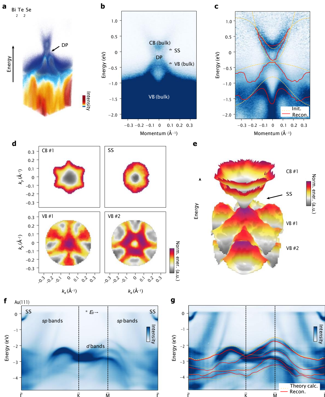
Fig. 6 | Band reconstruction for \text{Bi}_2\text{Te}_2\text{Se} and \text{Au}(111) . a , 3D view of the photoemission band-mapping data of the topological insulator \text{Bi}_2\text{Te}_2\text{Se} around the Dirac point (DP). b , The energy bands near the DP are labeled in a 2D data slice through the DP. CB, conduction band; VB, valence band; SS, surface state. c , The outcome of reconstruction (after smoothing) is superimposed on the pre-processed data. d,e , Momentum-resolved reconstruction, shown in 2D
