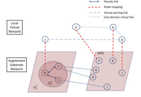
Fig. 4: downsizing link mapping by InP_2
