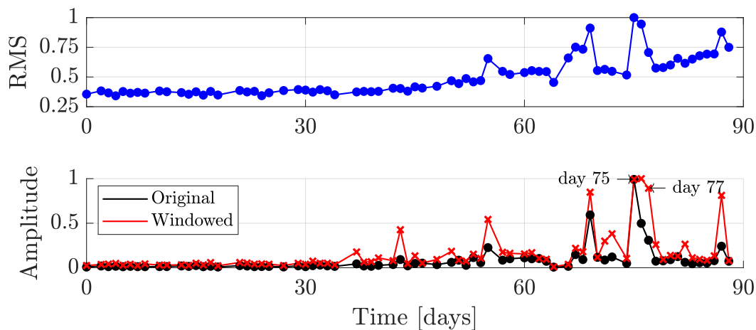
Figure 8: Scalar indicator calculated from 10s vibration acquisition during a period of three months. The root mean square of the signal is presented (top) along with the maximum amplitude of the spectrum within a narrow band around the expected fault frequency (bottom).
