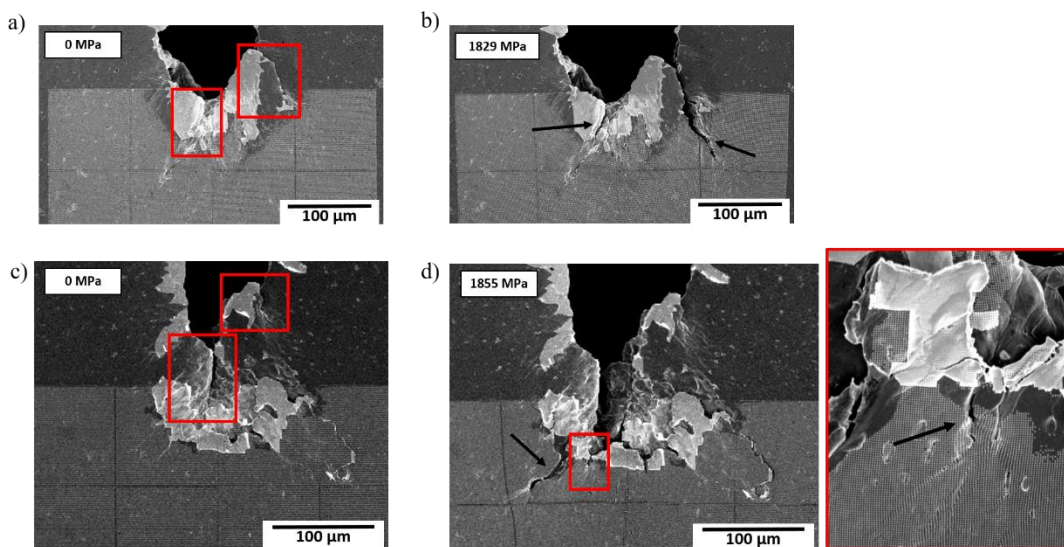
Fig. 7. SEM images of (a) SMATed sample 1 at initial state; (b) SMATed sample 1 at 1829 MPa; (c) SMATed sample 2 at initial state; (d) SMATed sample at 1855 MPa with a magnification zone.
