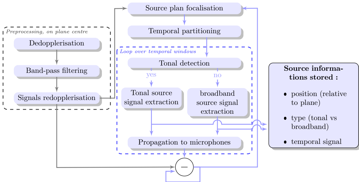
Figure 1: CleanT algorithm applied to the flyover antenna. Black arrows are executed at startup only, blue arrows are borrowed at each iteration.
