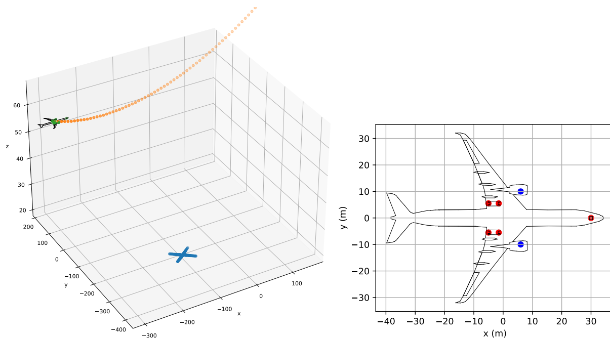
(a) Sources (in green) and aircraft at t = 0 , its trajectory (in orange) and the microphone array (in blue)
