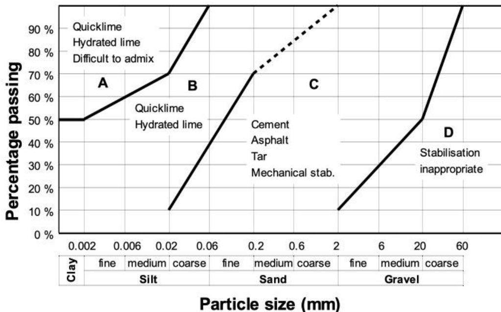
Figure 1. Recommended binders for different soil types (Assarsson, 1968). Note that tar is now classified as an environmental problem.
