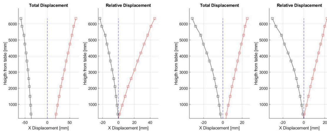
Fig. 10. Configuration 2: specimen total and relative displacement profiles corresponding to the attainment of the maximum acceleration intensities (0.136 g, Alkion accelerometer (left) and 0.101 g, Basso-Tirreno accelerometer (right)).
