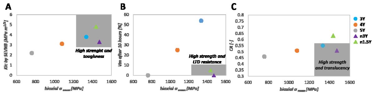
Figure 8 : Summary of the mechanical, optical and LTD resistance properties of the zirconia grades. In (A) the compromise between strength and toughness, in (B) the compromise between strength and LTD resistance and in (C) the compromise between strength and optical properties.
