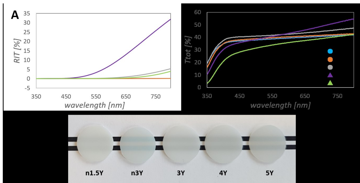
Figure 6 : Optical properties of the different zirconia grades. (A) Real In-line Transmission as a function of wavelength, (B) Total Forward Transmission as a function of wavelength and (C) optical images of 1 mm thick samples.
