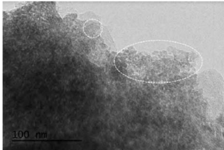
Fig. 5. TEM image of a few discrete spherical particles interpreted as allophanes (Okagawa, 1971; Hanmi and Wada, 1976; Parfitt, 1990) at the edges of clay particles (see in the circles) for the cultivated BS3 site. Spherical particles have a diameter of 6 nm and are composed of a disc with a white central part interpreted as being the projection of a hollow sphere. It was not possible to observe them individually and they are systematically associated with clay particles.
