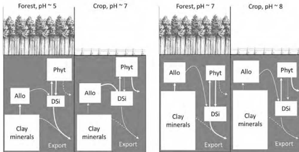
Fig. 8. Adaptation of the Struyf et al. (2010) conceptual model for the impact of land use change from mature forests to long-term cultivated areas on the main pools that control soluble Si in soils developed on loess (left-hand side) and calcareous soils (right-hand side). Boxes represent the main Si pools with the size of the boxes representing the relative size of the stock. Arrows represent fluxes with a thickness depending on their relative importance. Dashed arrows represent irrelevant fluxes. Ph, Si in phytoliths; DSi, soluble Si estimated by Si_{CaCl_2} ; Allo, Si in allophanes.
