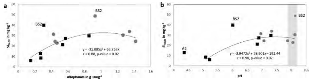
Fig. 7. Soluble Si ( Si_{CaCl_2} ) as a function of the allophane amount (a) and pH (b) in forest soils in black and cultivated soils in grey. Allophane content was calculated using Harsh's (2005) equation: % allophane = Si_e / (-0.067 Al_e / Si_e + 0.27) . The grey rectangle corresponds both to the point of zero charge of the allophanes and to the equilibrium with calcite. In both cases, the regression line was performed on all the soils that are not identified. Forest sites correspond to composite values (0–25 cm) calculated considering the thickness of the two sampled horizons (0–5 cm and 5–25 cm), their concentrations in the different elements and their respective bulk densities.
