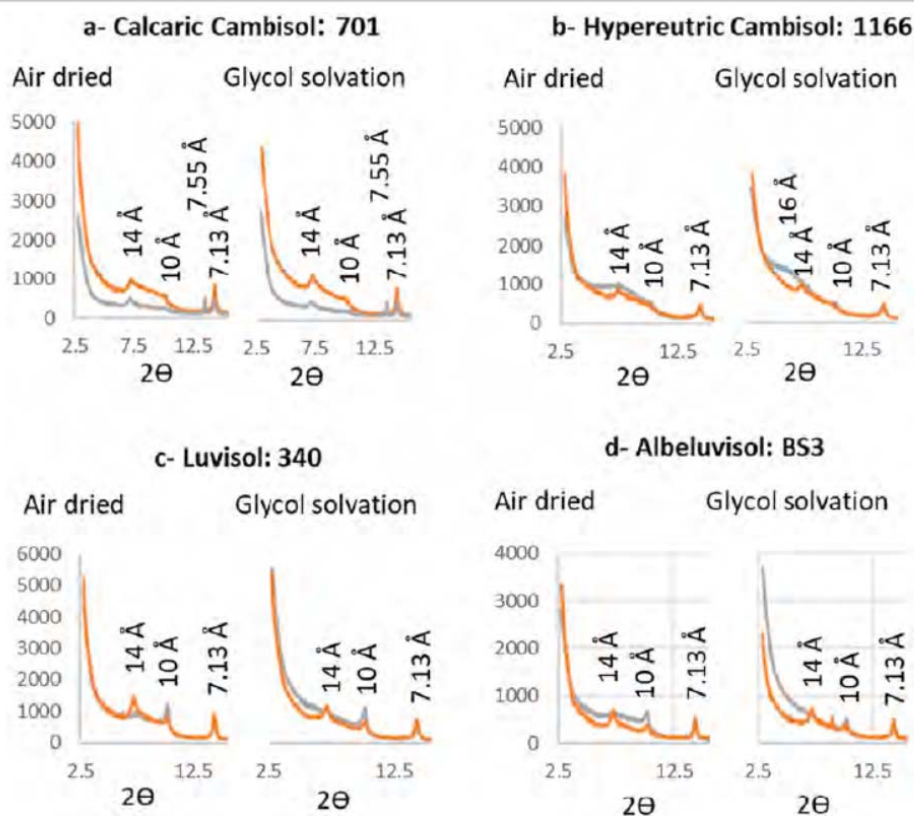
D patterns of the < 2 \mu\text{m}</math> fraction on oriented slides of the cultivated (in grey) and forest (in orange) soils: a- for the calcaric Cambisol 701; b- the c Cambisol 1166; c- the Luvisol 340; and d- the Albeluvisol.
