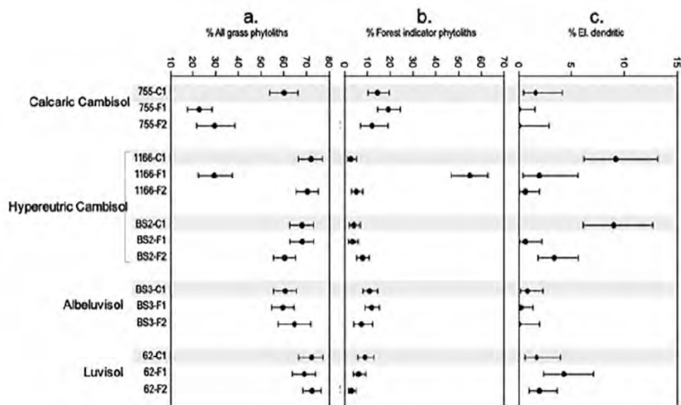
Fig. 3. Relative abundance of (a) grass phytoliths (including RONDEL, CREMATE, ELOBATE, POLYLOBATE, and CROSS silica short cells, silicified epidermal tissues, FLABELLATE BULLIFORM cells, and ELONGATE DENDRITIC), (b) forest indicator phytoliths (including SPHEROIDS, sclereids and other silica bodies observed in woody dicotyledons, two BLOCKY FACETED bodies typical of conifers, and a very long and large ELONGATE phytolith typical of some ferns (see details in S1 Table-Phyto). (c) Relative abundance of ELONGATE DENDRITIC phytoliths typical of grass inflorescences. Bars represent 95% confidence intervals. Percentages were calculated based on (a, b) total sum of particles counted and (c) on total phytolith sum.
