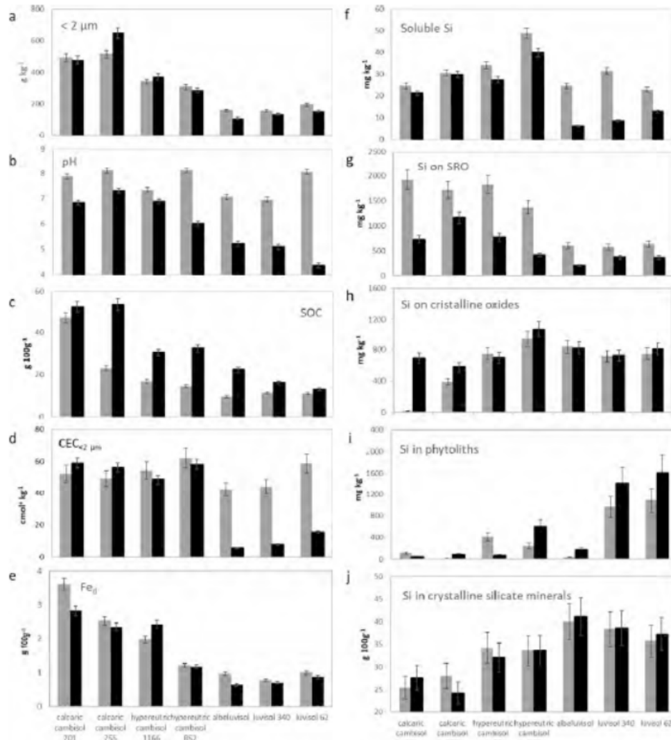
Fig. 2. < 2 \mu\text{m} fraction (a), pH (b), SOC (c), CEC of the < 2 \mu\text{m} fraction (d) and the Fe in iron oxides ( \text{Fe}_\text{o} ; e), and different Si forms (f: soluble and bioavailable Si ( \text{Si}_{\text{CaCl}_2} ); g: Si in SRO minerals ( \text{Si}_\text{s} - \text{Si}_{\text{CaCl}_2} ); h: Si in crystalline Fe oxides ( \text{Si}_\text{c} - \text{Si}_\text{o} ); i: Si in phytoliths; j: Si in crystalline silicate minerals ( \text{Si}_{\text{sil}} - \text{Si}_\text{d} )) in cultivated (in grey) and forest (in black) soils of the paired sites studied. Forested sites correspond to composite values (0–25 cm) calculated considering the thickness of the two sampled horizons (0–5 cm and 5–25 cm), their concentrations in the different elements and their respective bulk densities. Error bars correspond to the analytical uncertainties.
