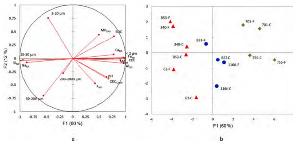
Fig. 1. Principal component analysis (PCA) of the pedological characteristics and major element concentrations for the seven paired sites studied. a- Circle of correlations; b- space of the individuals (F states for forest and C for cultivation). Different symbols correspond to the different groups defined by a hierarchical classification performed on the first two factors of the PCA. Green diamonds encompass the calcaric Cambisols, blue circles the hypereutric Cambisols and red triangles correspond to soils developed on loess parent materials. Forest sites correspond to composite values (0–25 cm) calculated considering the thickness of the two sampled horizons (0–5 cm and 5–25 cm), their concentrations in the different elements and their respective bulk densities.
