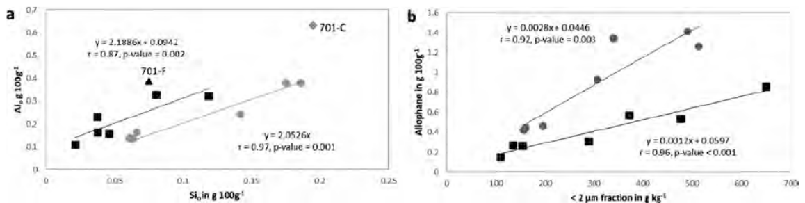
Fig. 6. Impact of land use on the allophane amount in the paired-sites: a- Al_0 as a function of Si_0 ; b- amount in allophanes as a function of the < 2 \mu m concentration. Allophane content was calculated using Harsh's (2005) equation: % allophane = Si_0 / (-0.067 Al_0 / Si_0 + 0.27) . Forest soils are reported in black and the cultivated soils in grey. Pearson correlation coefficient and p -values provided on the figures were calculated excluding the samples identified by their name (for figure a only). Forested sites correspond to composite values (0-25 cm) calculated considering the thickness of the two sampled horizons (0-5 cm and 5-25 cm), their concentrations in the different elements and their respective bulk densities.
