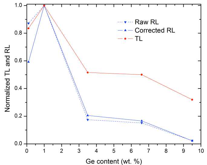
Fig. 5. Evolution of normalized TL and RL signal intensities as a function of Ge content in the five fibers. The corrected RL values consider the correction factor f_c in Table 1.
