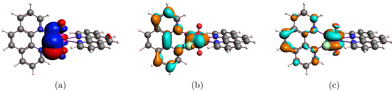
Figure 2: Molecular spinors: (a) occupied orbital from which the electron is excited; (b) empty orbital accepting the electron in the first three excited states; (c) empty orbital accepting the electron in the fourth excited state. Isosurface values are \pm 0.03 au.
