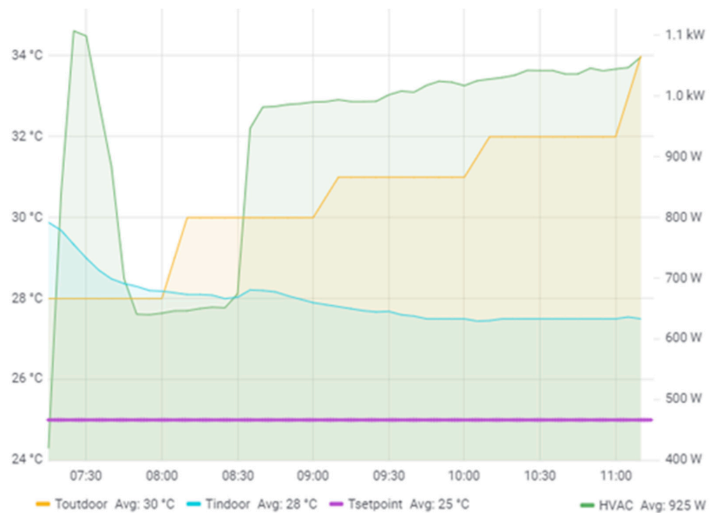
Figure 13. Experiment on the second day (Tsetpoint = 25 °C).
