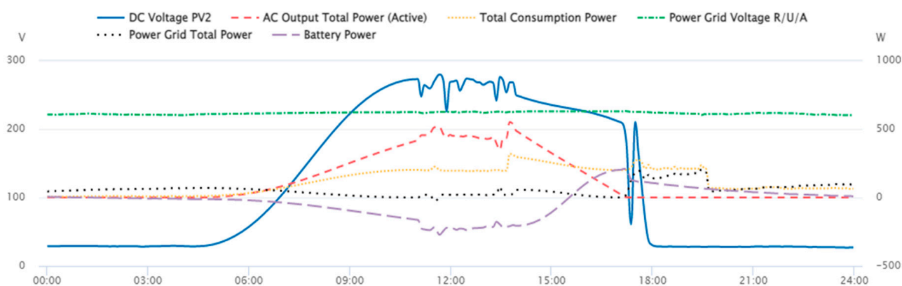
Figure 16. Power flows through inverter in 4 November 2021.
