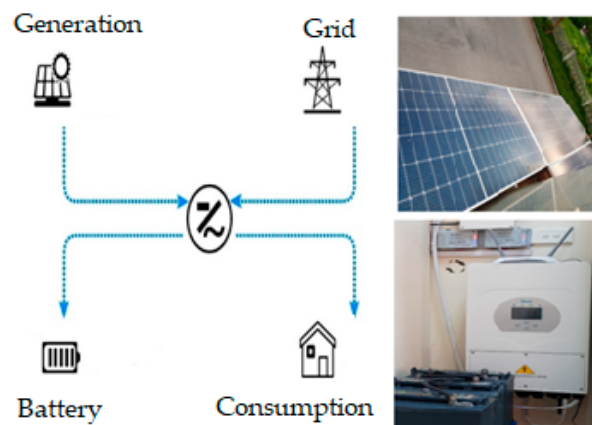
Figure 5. A demonstration of PV system in VHH's project.
