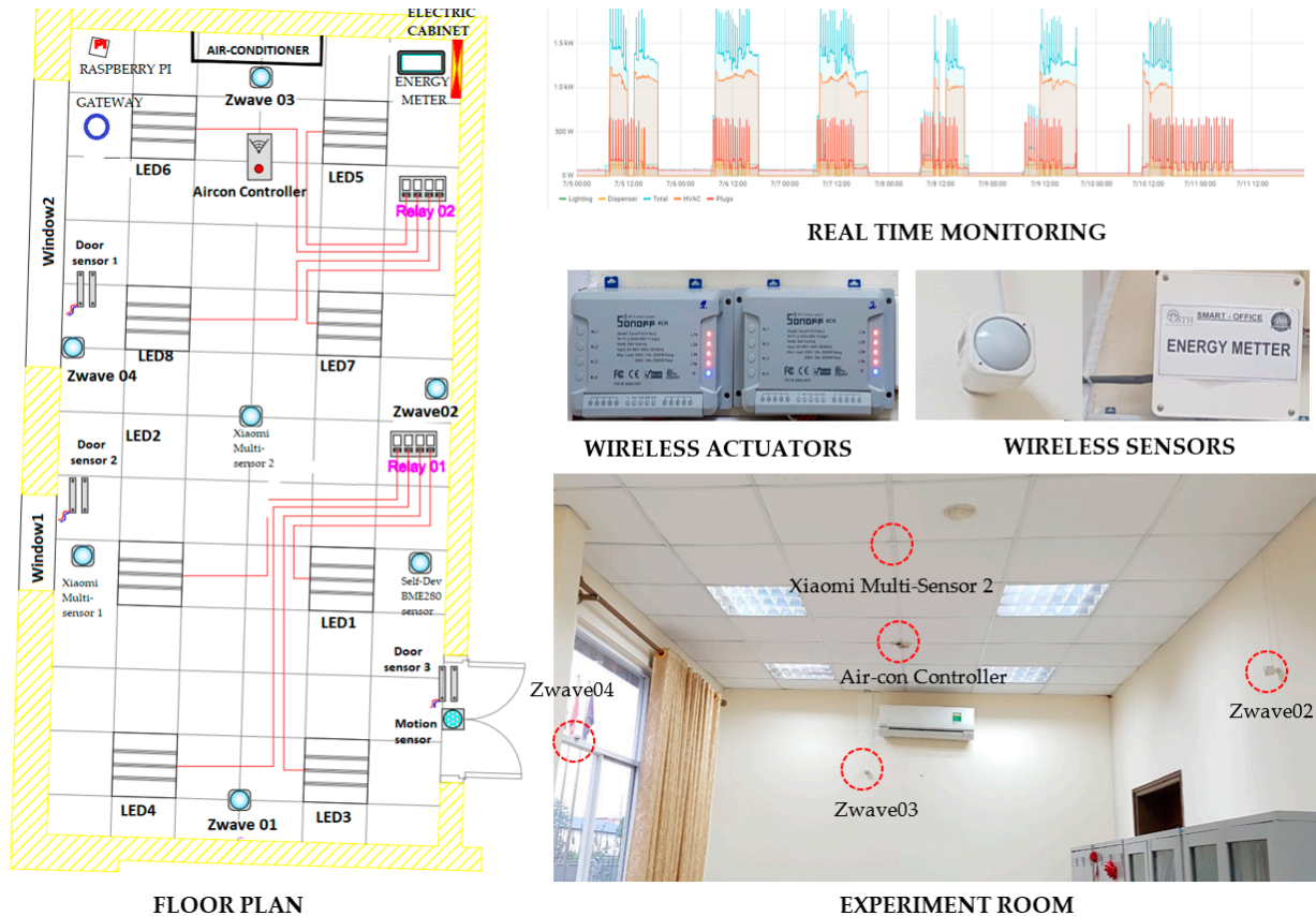
Figure 6. A demonstration of the wireless sensor and actuator networks (WSANs) in experiment room.
