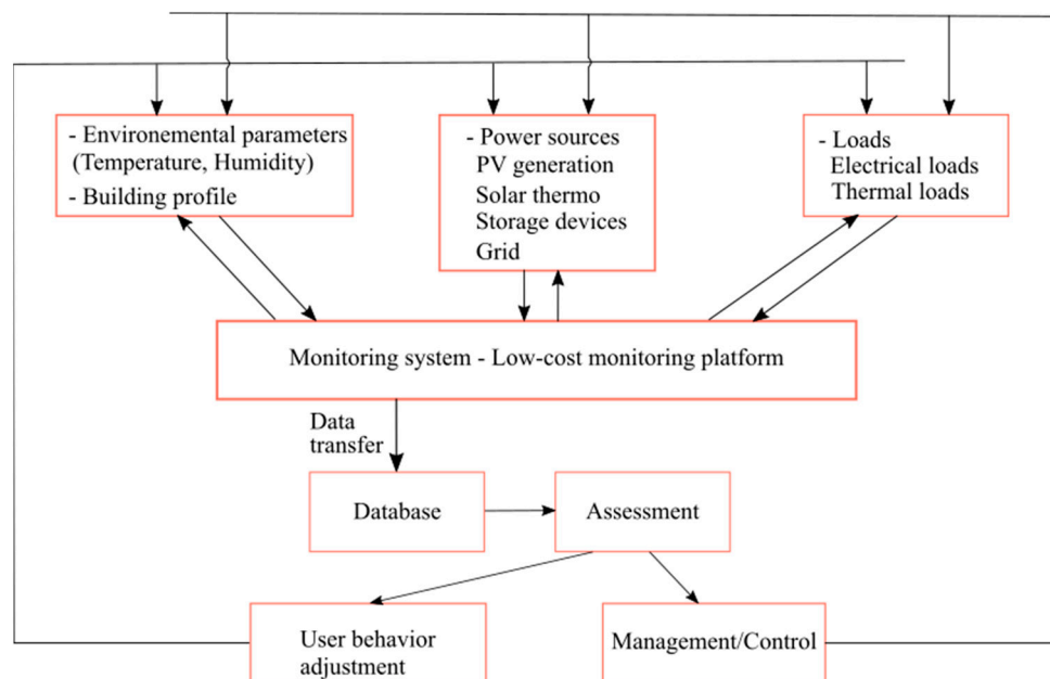
Figure 1. Schematic of energy efficiency management and role of monitoring platform.
