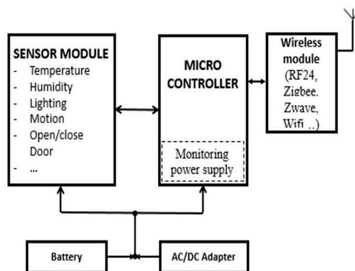
Figure 3. Overview of wireless sensor architecture.
