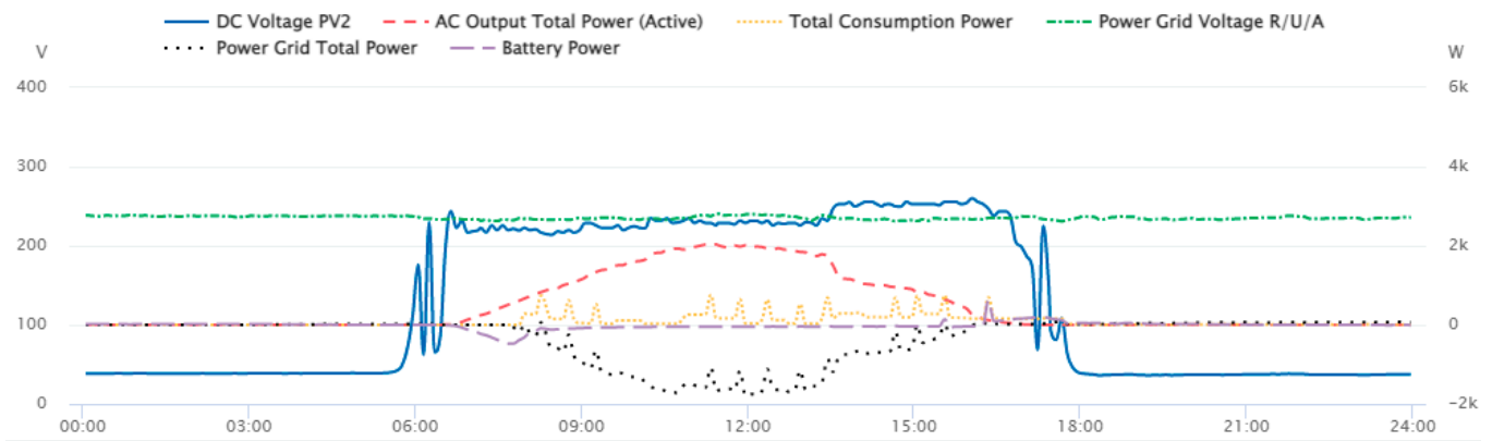
Figure 15. Power flows through inverter on 3 December 2021.
