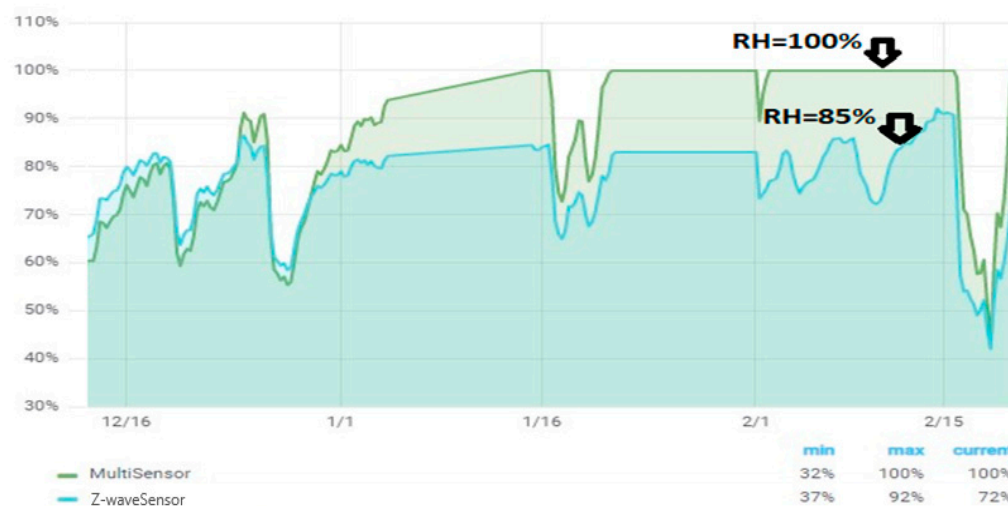
Figure 8. Operation of two sensors from 16 December 2019 to 15 February 2020.
