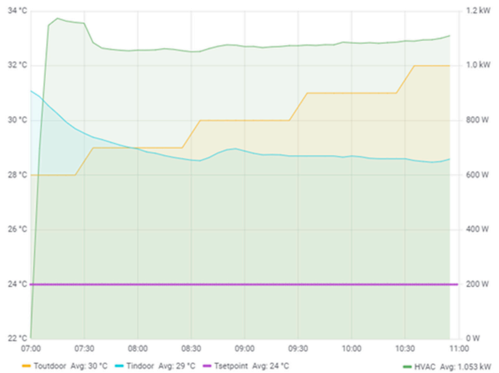
Figure 12. Experiment the first day (Tsetpoint = 24 °C).
