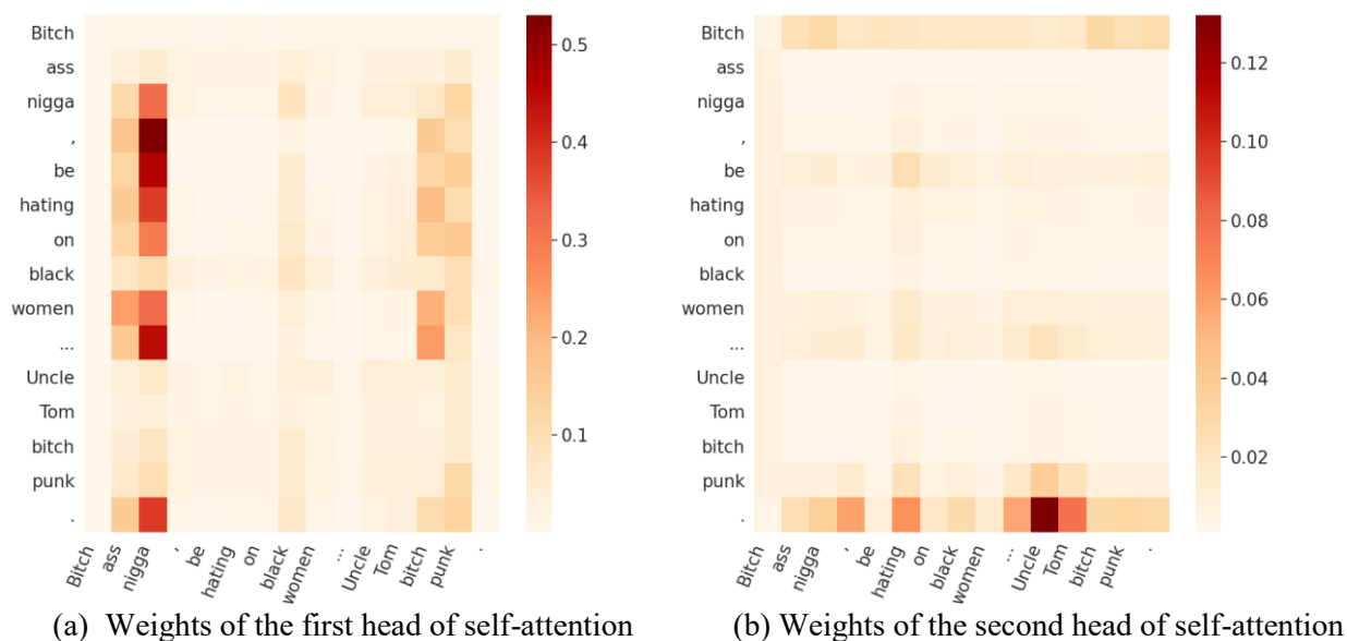
Fig. 2: Attention weights of the multi-task system with two heads (a and b) and the BERTweet embeddings. Example from the Davidson development set: “ Bitch ass nigga, be hating on black women... Uncle Tom bitch punk. ”. Two MWEs are detected: Bitch ass nigga and Uncle Tom .
