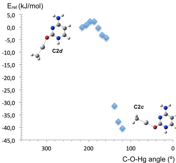
Figure S7. Plot of electronic energy values associated to the scan of the C2-O-Hg angle through the molecular plane from rotamer C2d to rotamer C2c (global minimum).
