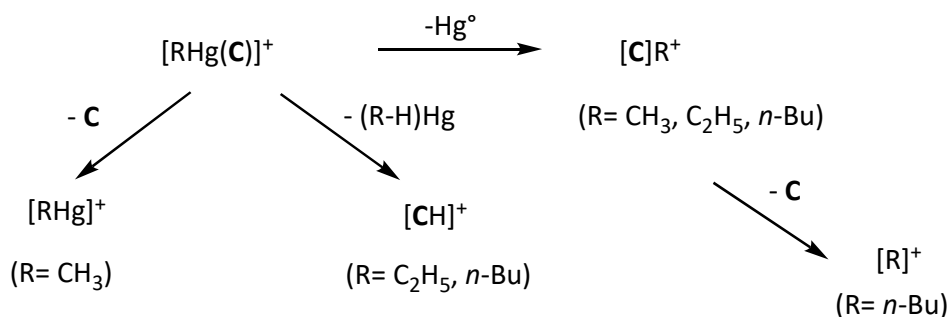
Scheme 1: fragmentation pattern of the [\text{RHg}(\text{C})]^+ complexes.
