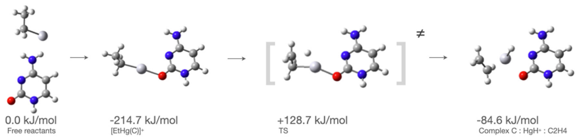
Figure S5. Transition state of a beta-hydride mechanism connecting [\text{EtHg}(\text{C})]^+ and product ( C : \text{HgH}^+ : \text{C}_2\text{H}_4 ) at the B3LYP/6-31++G(d,p)/def2-TZVPPD level of theory.
