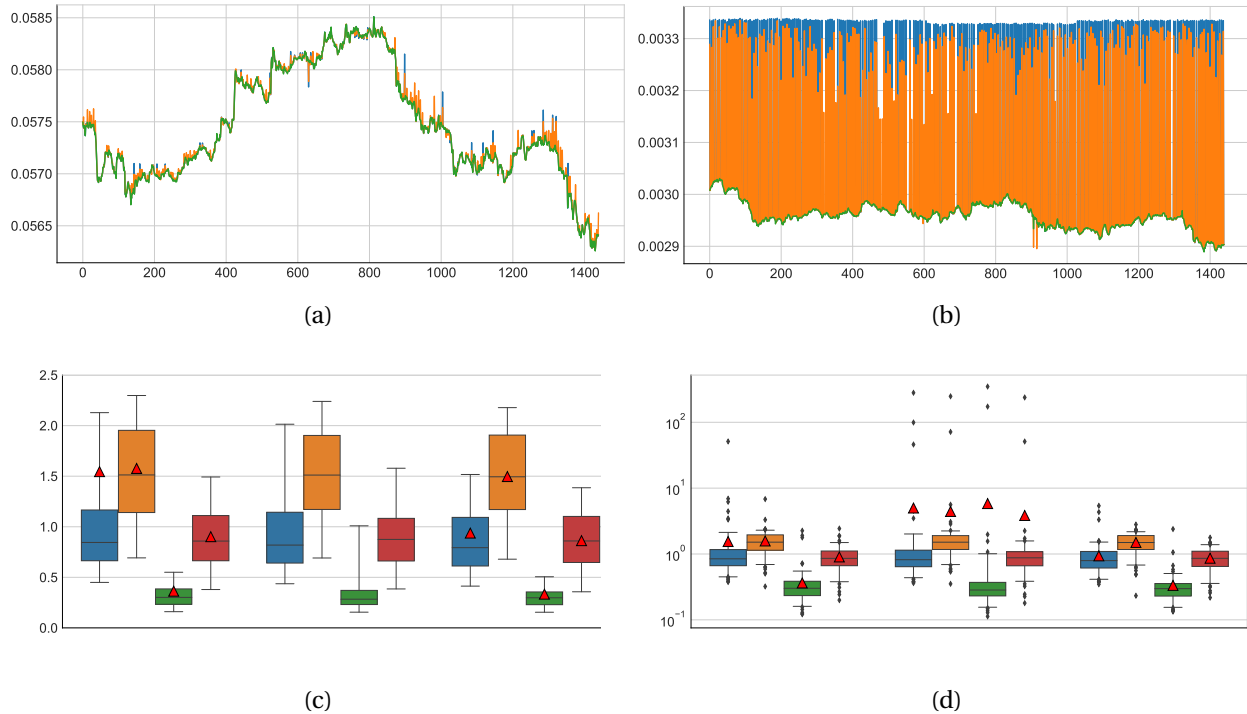
Figure 4: (a)-(b): Comparison between \widehat{VWM}_n (blue), \widehat{VWAP}_n (orange) and \widehat{RWM}_n (green) on real data aggregation per minute of the pair eth/btc (a) and zec/btc (b) on 2022-06-28. (c): Box plot of the annualized RV (over all pairs) from \widehat{VWM}_n (left), \widehat{VWAP}_n (middle) and \widehat{RWM}_n (right) on 2022-06-28 (blue), on 2022-06-12 (orange), on 2022-09-12 (green) and on 2022-05-05 (red). The mean is emphasized by a red triangle and outliers are discarded. (d) Box plot of the annualized RV taking into account outliers with the y-axis in log-scale.
