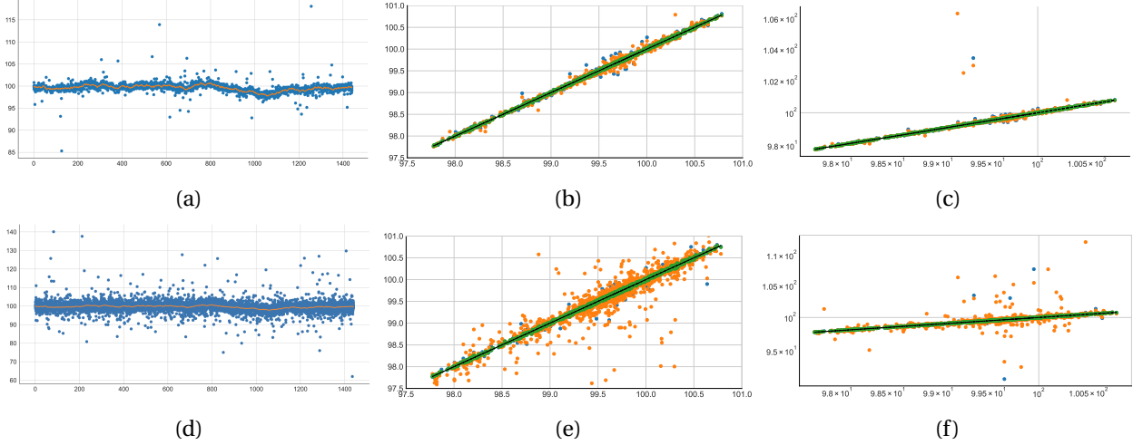
Figure 3: (a)-(d): Efficient price time-series (S_t)_{t=1}^{1440} (orange line) simulated with \sigma = 0.5 ( \sigma^{eff} = 0.51 ), and its associated noisy prices (\tilde{S}_t^j, j \in \{1, \dots, 100\})_{t=1}^{1440} (blue dots) with \omega = 0.99 (a) and \omega = 0.7 (d). (b)-(e): Scatter plots of the associated estimated prices (\hat{S}_t)_{t=1}^{100} ( \widehat{VWM}_n : blue, \widehat{VWAP}_n : orange, \widehat{RWM}_n : green) with respect to the reference price. The best estimator is illustrated by the black dashed regression line x \mapsto y = x . Both horizontal and vertical axes are limited to 97.5 and 101 for a better display. (c)-(f): Scatter plots of the reference price estimation with log-scale axes.
