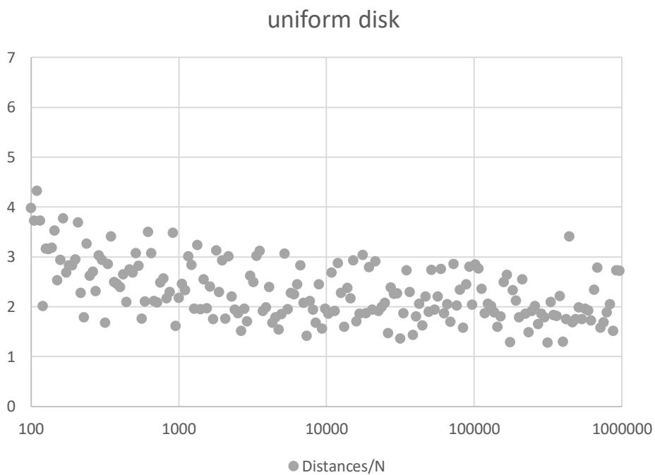
Figure 2. Ratio of the total number of distances computed over N , as a function of the size N of the set (semi-log scale). For large sets, this number is close to 2N .
