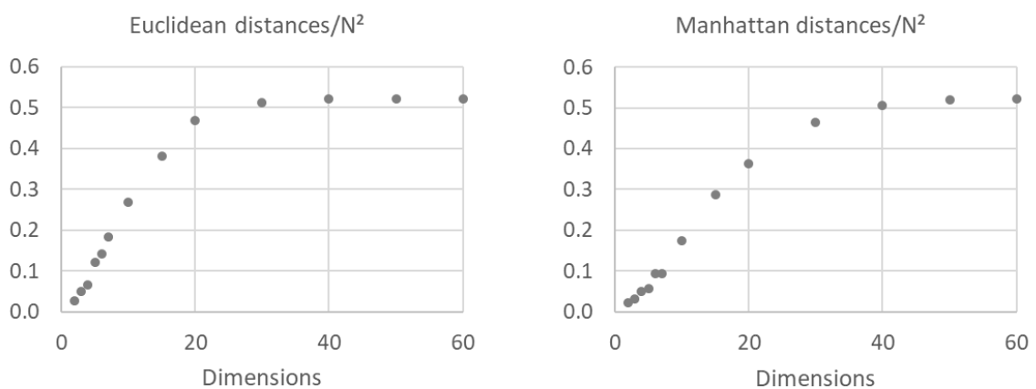
Figure 5. Ratio of the total number of distances computed over the square of the number of points N^2 , as a function of the number of dimensions (N in range 100 to 1000). For higher dimensions, the number of distance calculations increased quadratically and was close to N^2/2 , equivalent to the brute force method.
