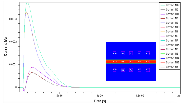
Fig. 8. 5x3 matrix. Comparison of currents at the fifteen contacts, LET=0.07pC/ \mu\text{m} , space=0.5 \mu\text{m} , depth=0.8 \mu\text{m} .
