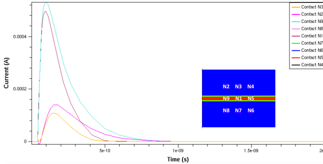
Fig. 5. 3x3 matrix. Comparison of currents at the nine contacts, LET=0.07pC/ \mu\text{m} , space=0.5 \mu\text{m} , depth=0.8 \mu\text{m} .
