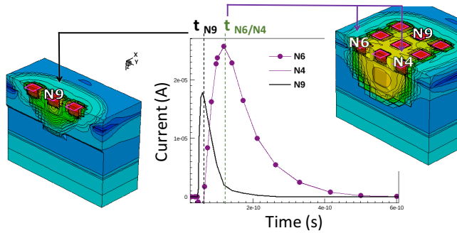
Fig. 13. Current versus time at three contacts: N9, N6 and N4 – alpha particle case.
