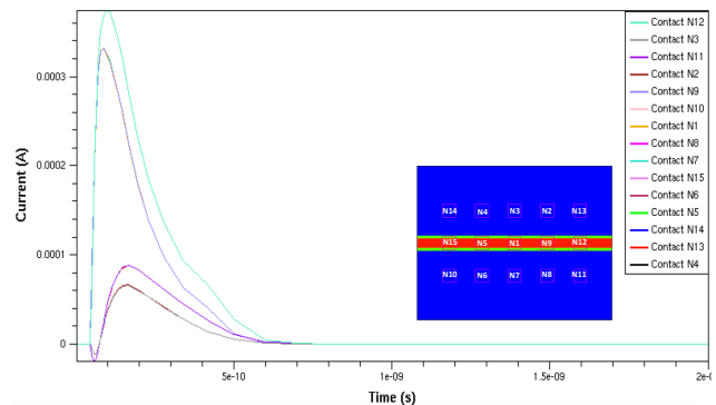
Fig. 8. 5x3 matrix. Comparison of currents at the fifteen contacts, LET=0.07pC/ \mu\text{m} , space=0.5 \mu\text{m} , depth=0.8 \mu\text{m} .
