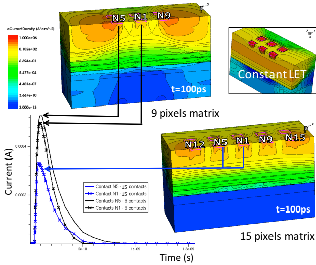
Fig. 10. Comparison of N1 and N5 currents of the 3x3 and 5x3 matrix, LET=0.07pC/μm, space=0.5μm, depth=0.8μm.
