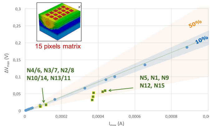
Fig. 18. Linearity curve and detected currents concerning an aluminum ion crossing in a fifteen contacts matrix.
