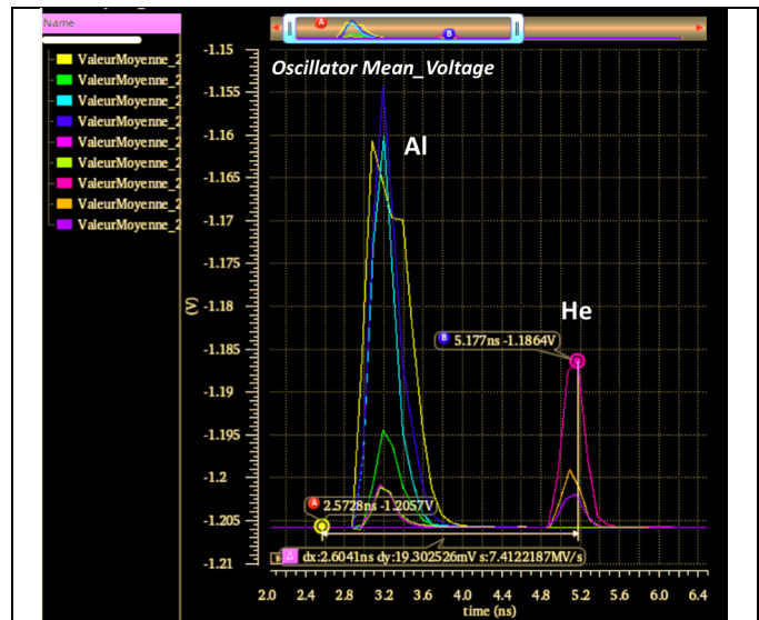
Fig. 27. Mean voltage for the highest currents: aluminum on the left, alpha on the right.
