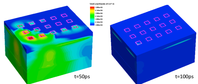
Fig. 22. Total current density at t=50ps (maximum of the generation) and t=100ps for the alpha particle.
