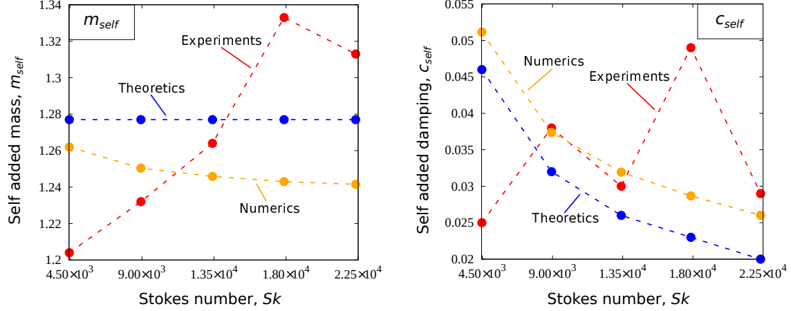
Figure 13: Study 2. Evolution of the self-added coefficients with the Stokes number Sk , for P/D = 1.5 and KC = 10^{-1} . The red, blue and orange dashed lines with points refer respectively to the experimental measurements, the theoretical estimations of [53] and the numerical predictions.
