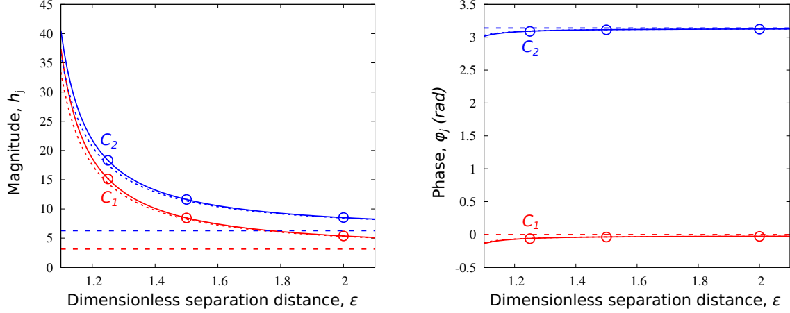
Figure 5: Study 1. Evolution of the magnitudes h_j and phases \varphi_j with the dimensionless separation distance \varepsilon , for Sk = 10^4 and KC = 10^{-2} . The red and blue solid lines correspond to the theoretical estimations of [50], see Eq. (16). The dashed lines correspond to the theoretical asymptotic expansion Sk \rightarrow \infty , see Eq. (18). The horizontal dashed lines correspond to the theoretical isolated cylinder limits as \varepsilon \rightarrow \infty . The symbols correspond to the numerical predictions.
