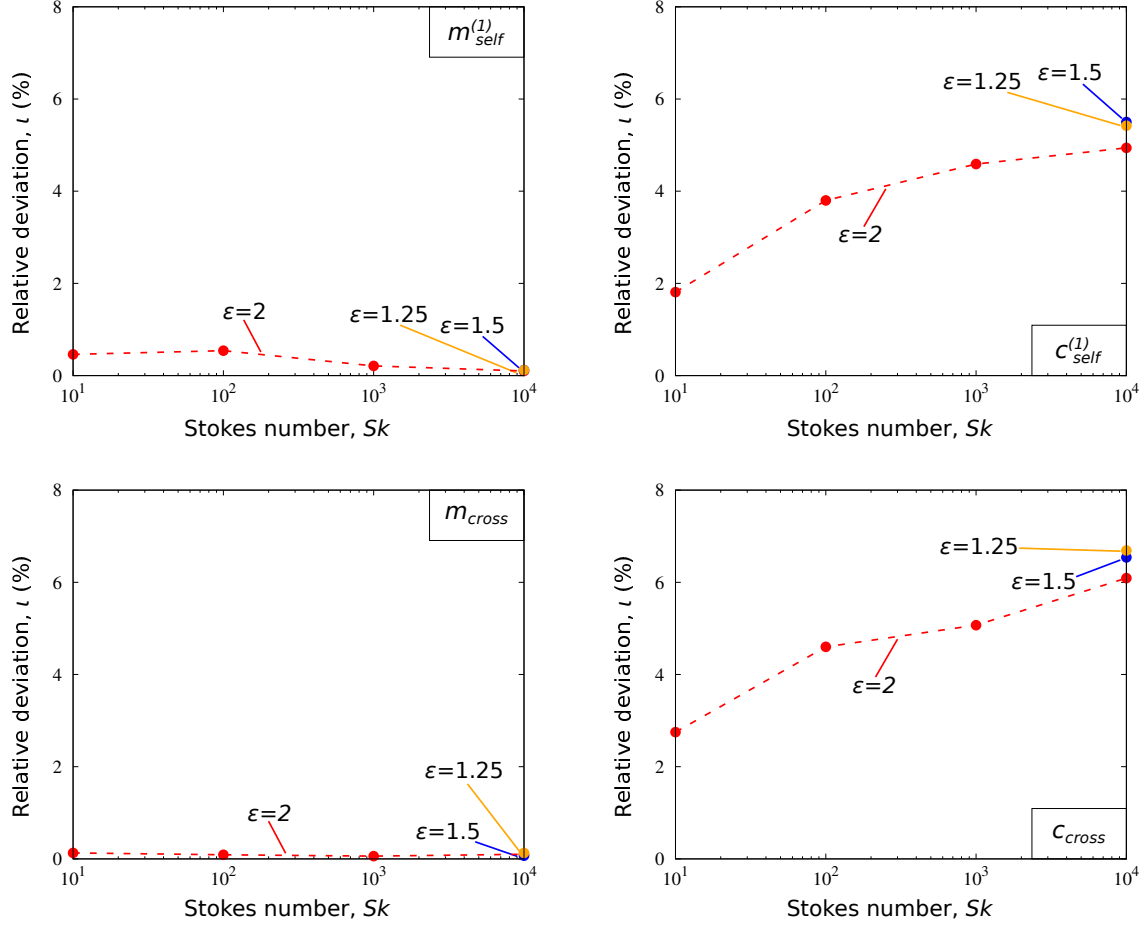
Figure 8: Study 1. Evolution of the relative deviation, \iota with the Stokes number, Sk for different value of \epsilon and KC = 10^{-2} . The red dotted lines with points refer to \epsilon = 2 , the blue points refer to \epsilon = 1.5 while the orange points refer to \epsilon = 1.25 .
