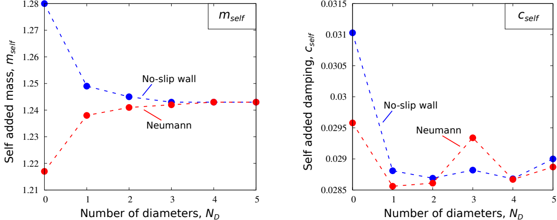
Figure 11: Study 2. Evolution of the self-added coefficients with the size of the fluid domain (the size of the fluid domain increases by a distance of N_D diameters in the y -directions). The blue (resp. red) dashed line corresponds to the numerical predictions obtained with a wall boundary condition (resp. a Neumann boundary condition) imposed on the top and bottom boundaries of the computational domain, see Fig. 10. The dimensionless parameters are Sk = 1.8 \times 10^4 , P/D = 1.5 and KC = 10^{-1} .
