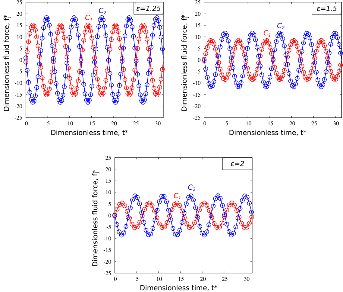
Figure 3: Study 1. Time evolution of the dimensionless fluid forces, for \epsilon = \{1.25, 1.5, 2\} , Sk = 10^4 and KC = 10^{-2} . The red and blue solid lines correspond to the theoretical estimations of [50], see Eq. (16). The symbols correspond to the numerical predictions.
