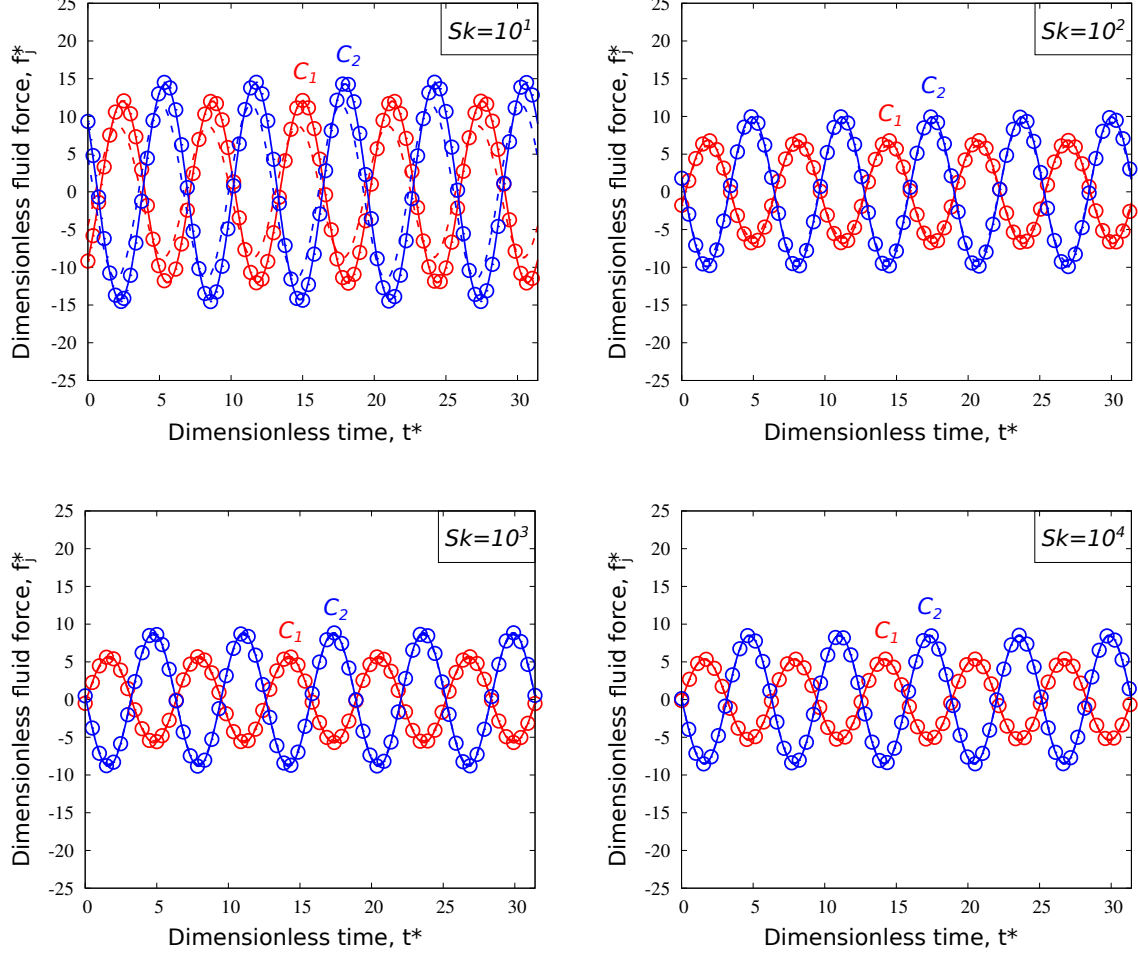
Figure 2: Study 1. Time evolution of the dimensionless fluid forces, for Sk = \{10^1, 10^2, 10^3, 10^4\} , \varepsilon = 2 and KC = 10^{-2} . The red and blue solid lines correspond to the theoretical estimations of [50], see Eq. (16). The dashed lines (indistinguishable from the solid lines for Sk > 10^2 ) correspond to the theoretical asymptotic expansion Sk \rightarrow \infty , see Eq. (18). The symbols correspond to the numerical predictions.
