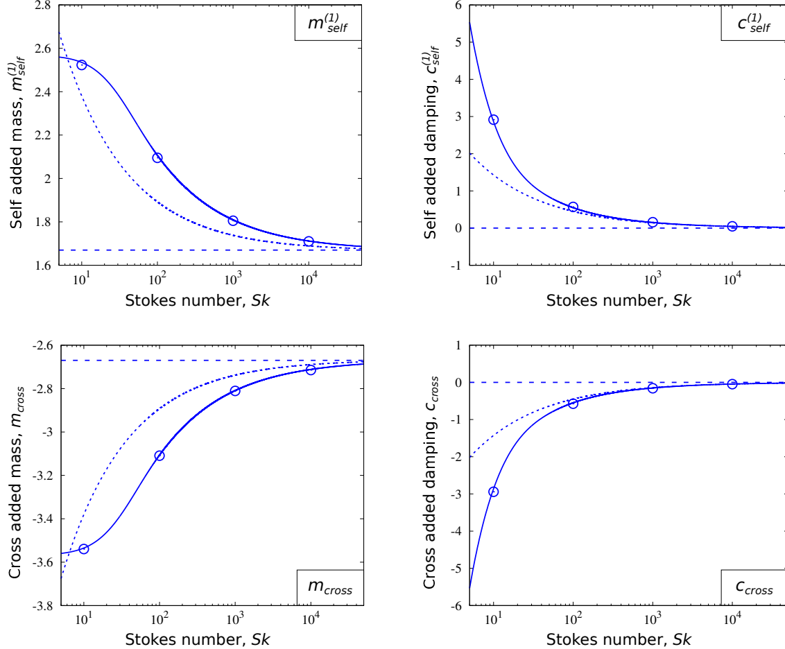
Figure 6: Study 1. Evolution of the added coefficients with the Stokes numbers Sk , for \varepsilon = 2 and KC = 10^{-2} . The solid lines refer to the theoretical estimations of [50], see Eq. (16). The dashed lines correspond to the theoretical asymptotic expansion Sk \rightarrow \infty , see Eq. (18). The horizontal dashed lines correspond to the theoretical inviscid limits as Sk \rightarrow \infty . The symbols correspond to the numerical predictions.
