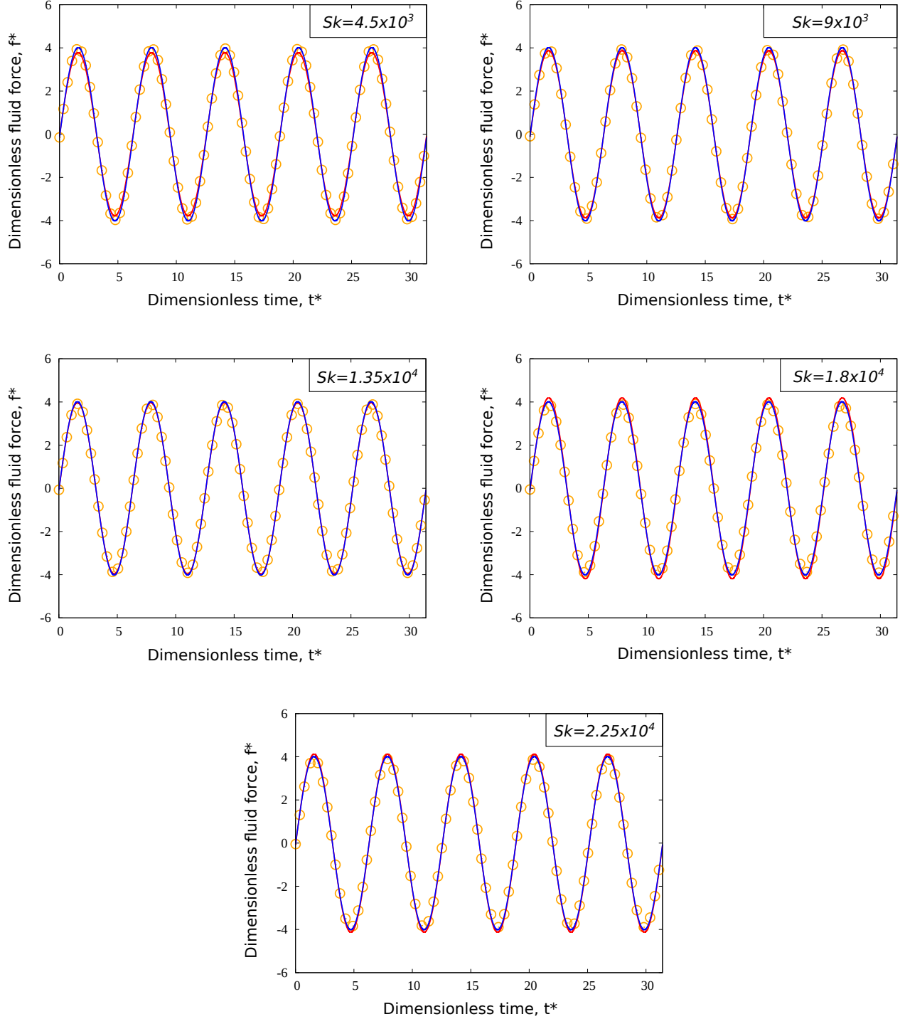
Figure 12: Study 2. Time evolution of the dimensionless fluid forces, for Sk \in \{0.45, 0.90, 1.35, 1.80, 2.25\} \times 10^4 , P/D = 1.5 and KC = 10^{-1} . The blue solid lines correspond to the theoretical estimations of [53], see Eq. (23). The red solid lines correspond to the experimental measurements. The orange symbols correspond to the numerical predictions. (For interpretation of the colors in this figure, the reader is referred to the web version of this article).
