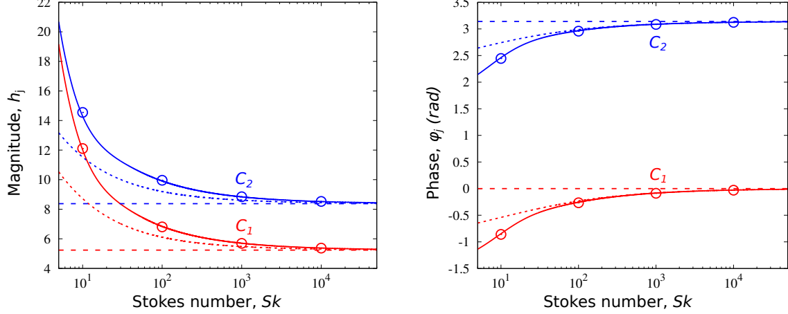
Figure 4: Study 1. Evolution of the magnitudes h_j and phases \varphi_j with the Stokes number Sk , for \varepsilon = 2 and KC = 10^{-2} . The red and blue solid lines correspond to the theoretical estimations of [50], see Eq. (16). The dashed lines correspond to the theoretical asymptotic expansion Sk \rightarrow \infty , see Eq. (18). The horizontal dashed lines correspond to the theoretical inviscid limits as Sk \rightarrow \infty . The symbols correspond to the numerical predictions.
