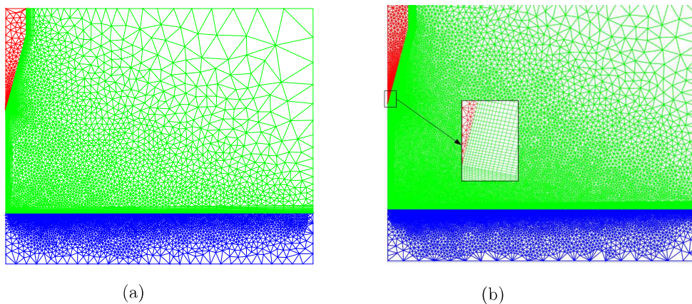
Figure 2: The meshes for the PNT \alpha = 15^\circ case. a) \mathcal{M}_1 : coarsest mesh with 15,487 elements b) \mathcal{M}_3 : finest mesh with 42,089 elements. The red, green and blue zones represent the meshes of the cathode, arc-plasma and anode, respectively.
