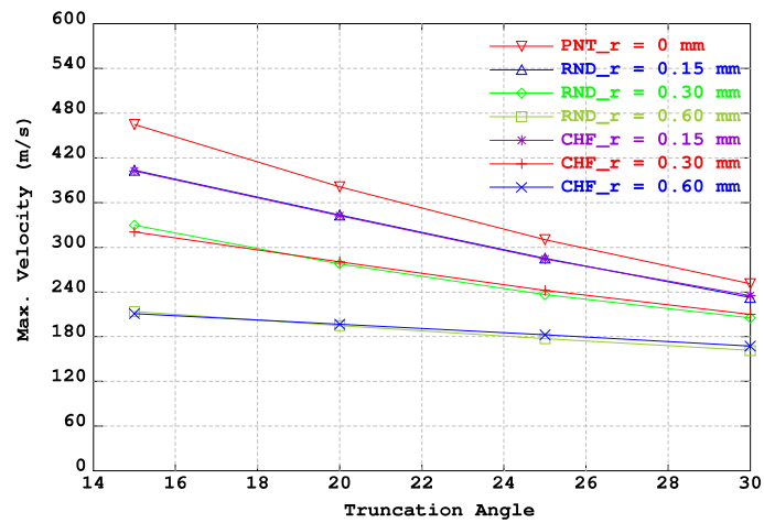
Figure 9: Maximum arc velocity versus truncation angle (in degrees) and tip type.
