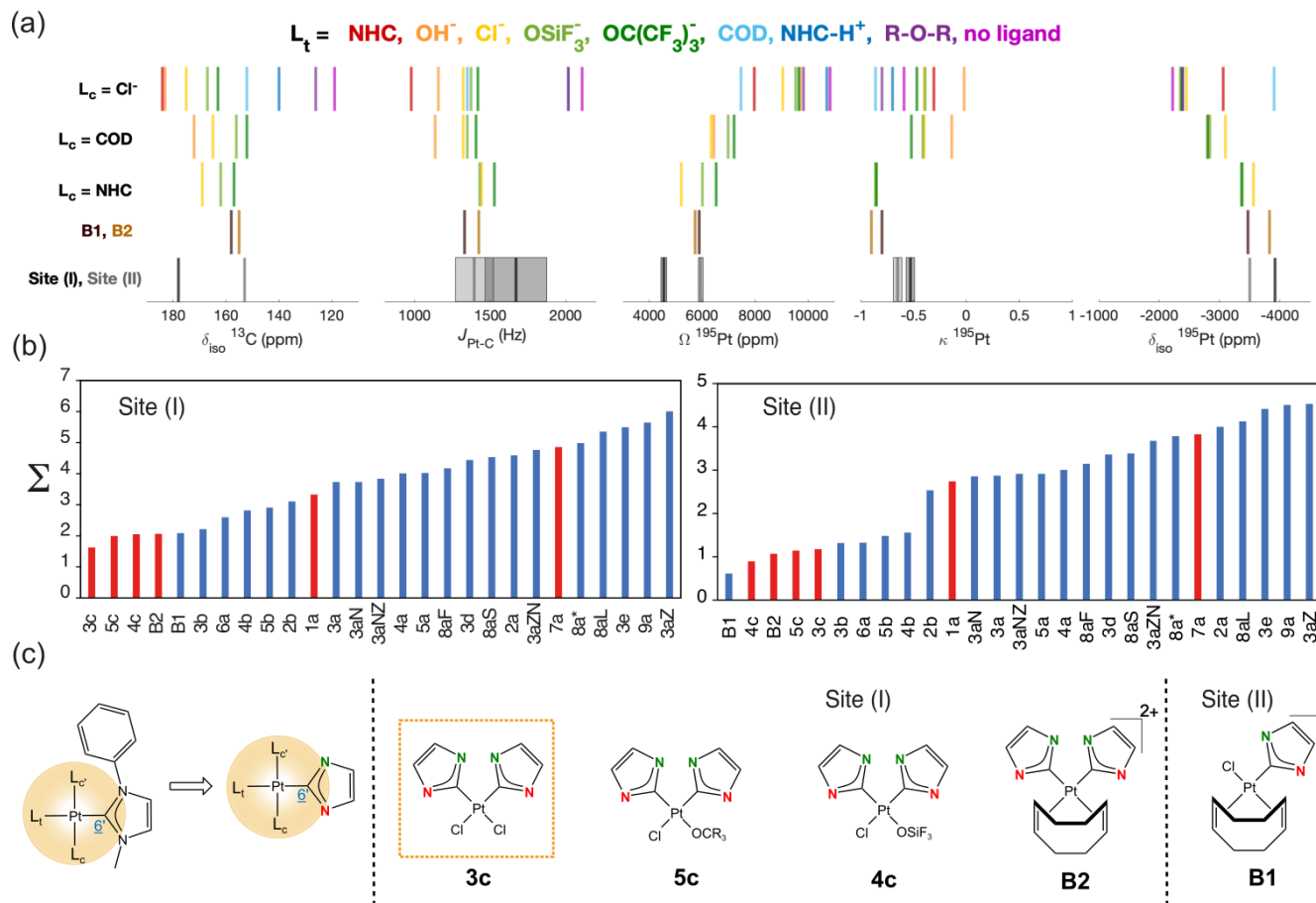
Figure 5. (a) “Barcode” representation of all evaluated NMR parameters; columns show from left to right: \delta_{\text{iso}}^{13}\text{C} , J(^{13}\text{C}-^{195}\text{Pt}) , \Omega^{195}\text{Pt} , \kappa^{195}\text{Pt} and \delta_{\text{iso}}^{195}\text{Pt} . The upper three rows show calculated values for compounds of type xn with L_c = \text{Cl}^- , COD and NHC respectively, while B1 and B2 are shown in the fourth row and the experimental data for site (I) and (II) in the fifth row. (b) Plot of the root-mean square deviation \Sigma as defined in the main text for the 27 molecular models. The red bars correspond to bis-NHC structures. (c) Most probable structural assignments for sites (I) and (II) based on the comparison between the experimental data and the DFT library of molecular model compounds. In the molecular models the two nitrogen atoms are bonded to a phenyl and a methyl group as represented in the left-hand side of the figure.
