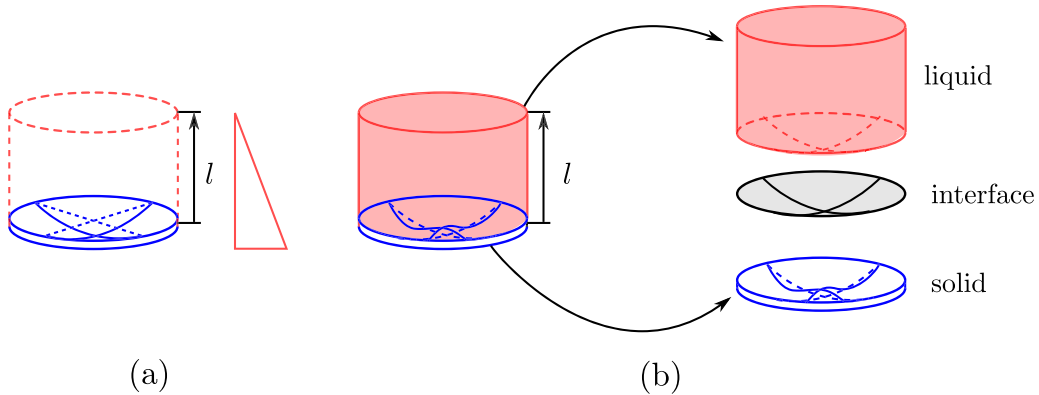
Fig. 9. (a) Prestressed state of the flexible bottom as a function of the liquid height l and (b) liquid–structure domains and interface.
