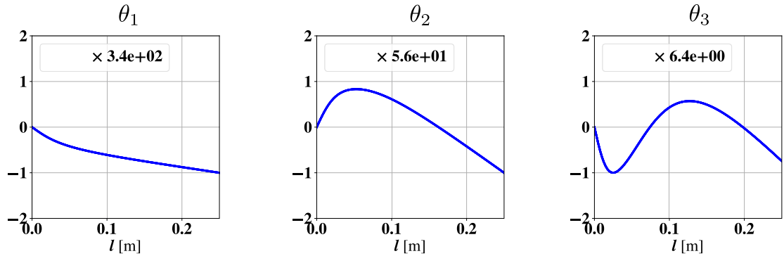
Fig. 11. Contributions of the reduced added mass matrices obtained via SVD as a function of the parameter l .
