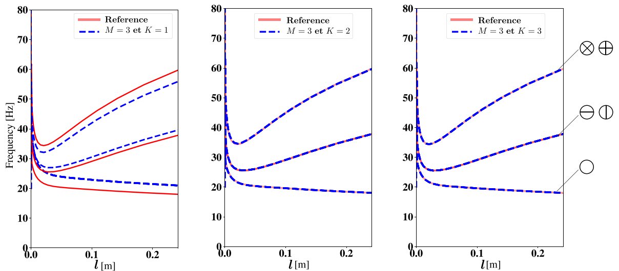
Fig. 12. Evolution of hydroelastic eigenfrequencies with prestress as a function of the loading parameter l for three reduced stiffness matrices \mathbf{K}_{i,i=1\dots 3} .
