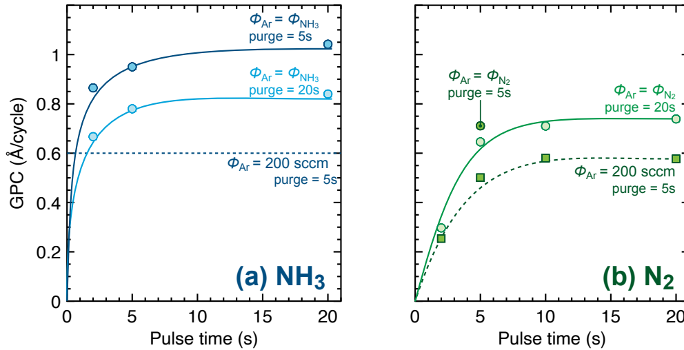
FIG. 6. (a) pl - NH_3 and (b) pl - N_2 pulses optimizations associate to purge duration. Circles and continuous lines correspond to equal flow conditions while squares and dashed lines stand for diluted conditions. The recipe used is 0.2:6:x_N:y_N s. N-source pulse times, x_N , correspond to abscissa while their purge times, y_N , are indicated on the plot.
