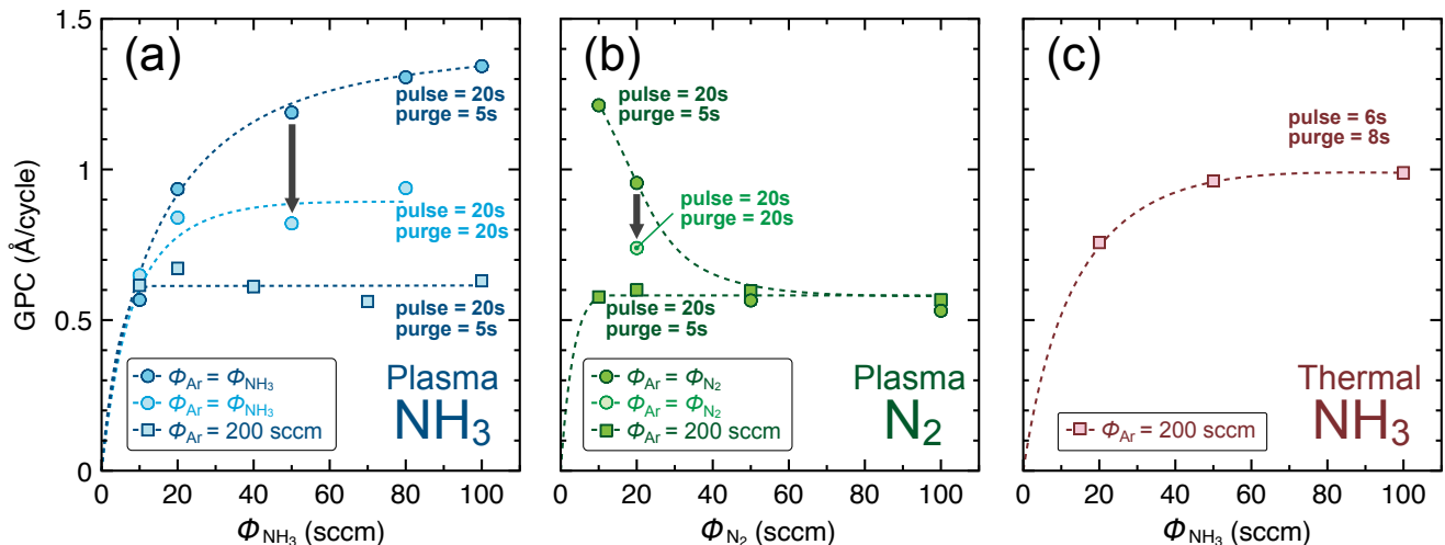
FIG. 3. Evolution of GPC depending on gas flow conditions for (a) pl -NH 3 and (b) pl -N 2 . GPCs are plotted against (a) \phi_{\text{NH}_3} and (b) \phi_{\text{N}_2} under diluted (squares) and equal flow (circles) conditions. Purge time is varied from 5 to 20 s in equal flow conditions for pl -NH 3 and pl -N 2 . (c) Evolution of GPC against \phi_{\text{NH}_3} under diluted conditions for the reference th -NH 3 process. In all cases, ALD sequence is 0.2:6: x_{\text{N}} : y_{\text{N}} ( x_{\text{N}} : y_{\text{N}} are indicated on the plots). Under diluted conditions \phi_{\text{Ar}} = 200 sccm.
