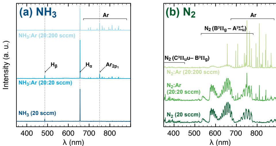
FIG. 4. OES spectra of (a) pl\text{-NH}_3 and (b) pl\text{-N}_2 pure or mixed within different Ar flows. Measurements are taken at the plasma generator window with P_{\text{plasma}} = 300 W using an acquisition time of 44 ms. The peaks have been identified according to literature 48–50 .
