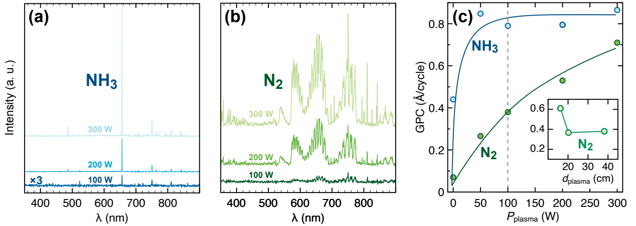
FIG. 7. OES spectra at different P_{\text{plasma}} for both (a) pl\text{-NH}_3 and (b) pl\text{-N}_2 mixed within Ar in equal flow conditions ( \phi_{\text{NH}_3} or \phi_{\text{N}_2} = \phi_{\text{Ar}} = 20 sccm and an acquisition time of 5 ms). Note that intensity of the pl\text{-NH}_3 spectrum at P_{\text{plasma}} = 100 W has been magnify ( \times 3 ) for better reading. (c) Influence of P_{\text{plasma}} on GPC for pl\text{-NH}_3 and pl\text{-N}_2 processes under equal flow conditions ( \phi_{\text{NH}_3} or \phi_{\text{N}_2} = \phi_{\text{Ar}} = 20 sccm). Inset shows the dependence of GPC against d_{\text{plasma}} for pl\text{-N}_2 at P_{\text{plasma}} = 100 W (corresponding to the vertical dashed line on the main plot).
