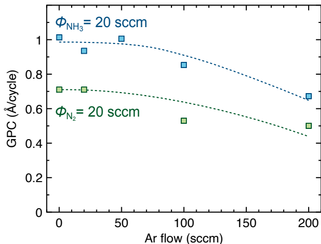
FIG. 5. Influence of dilution in Ar on both pl\text{-NH}_3 and pl\text{-N}_2 . \phi_{\text{NH}_3} and \phi_{\text{N}_2} are constant at 20 sccm.
