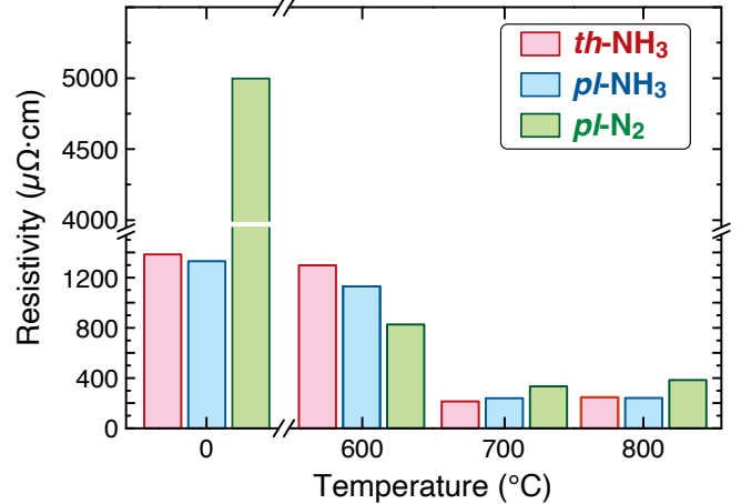
FIG. 13. Resistivity of TiN films grown by thermal- and PE-ALD (300 W, \phi_{\text{N-source}} = \phi_{\text{Ar}} = 20 sccm, P = 0.16 Torr) and effect of different annealings. TiN films were \approx 50 nm thick.
