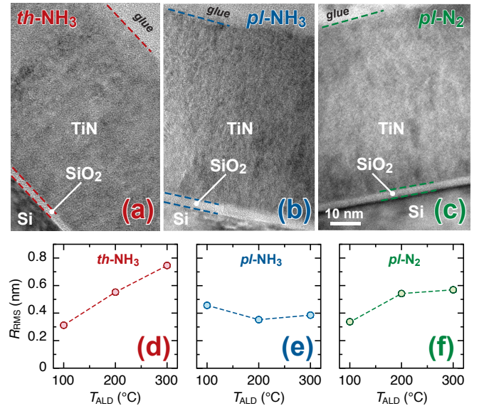
FIG. 8. TEM cross sections of TiN layers grown at T_{\text{ALD}} = 200^\circ\text{C} for (a) th\text{-NH}_3 , (b) pl\text{-NH}_3 and (c) pl\text{-N}_2 . R_{\text{RMS}} of TiN layers measured by AFM after N_{\text{ALD}} = 100 cycles depending on T_{\text{ALD}} for (d) th\text{-NH}_3 , (e) pl\text{-NH}_3 and (f) pl\text{-N}_2 .
