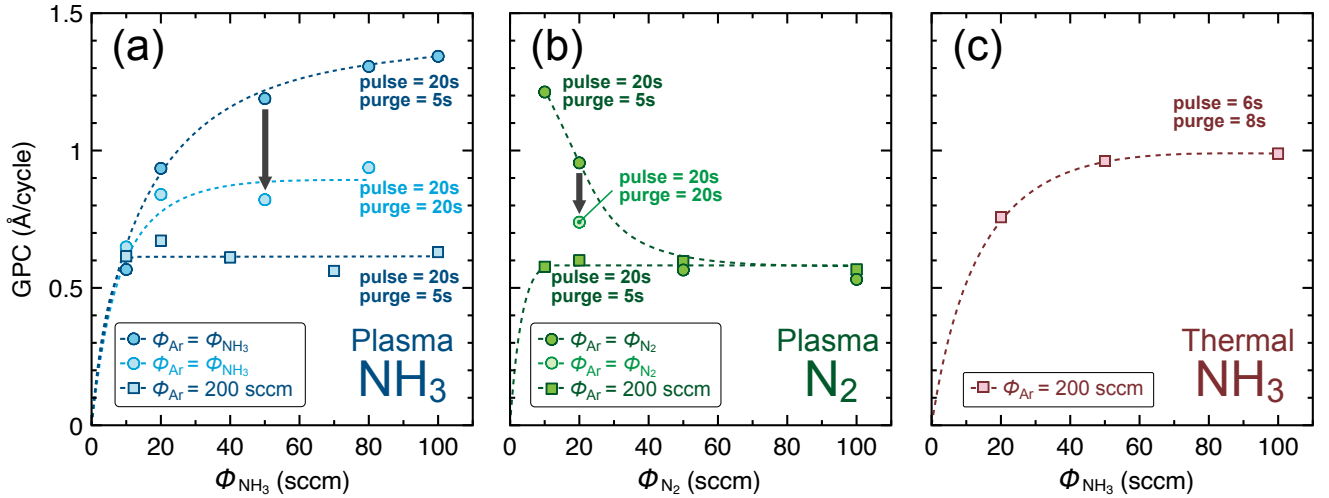
FIG. 3. Evolution of GPC depending on gas flow conditions for (a) pl -NH 3 and (b) pl -N 2 . GPCs are plotted against (a) \phi_{\text{NH}_3} and (b) \phi_{\text{N}_2} under diluted (squares) and equal flow (circles) conditions. Purge time is varied from 5 to 20 s in equal flow conditions for pl -NH 3 and pl -N 2 . (c) Evolution of GPC against \phi_{\text{NH}_3} under diluted conditions for the reference th -NH 3 process. In all cases, ALD sequence is 0.2:6: x_{\text{N}} : y_{\text{N}} ( x_{\text{N}} : y_{\text{N}} are indicated on the plots). Under diluted conditions \phi_{\text{Ar}} = 200 sccm.
