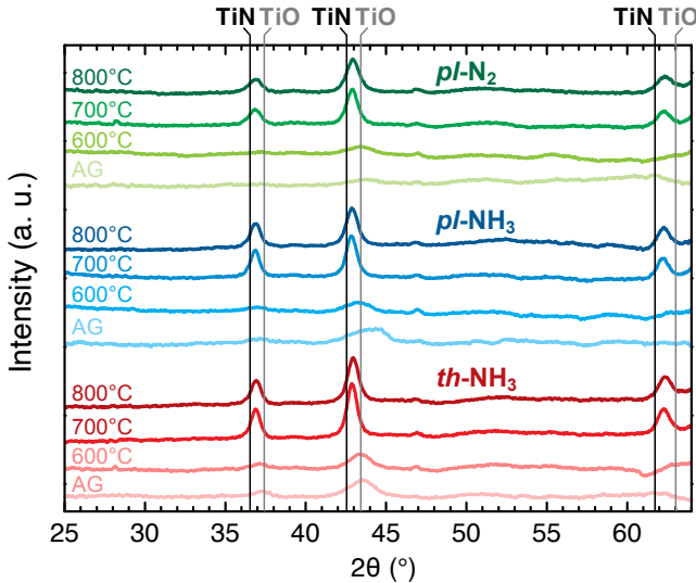
FIG. 12. XRD patterns of as-grown layers and their evolution with annealing temperature for the three deposition routes. Annealing in N 2 , NH 3 and H 2 mixture for 5 min at T_{\text{a}} = 600, 700 and 800^\circ\text{C} . Black and gray vertical lines correspond to TiN and TiO references, respectively.
