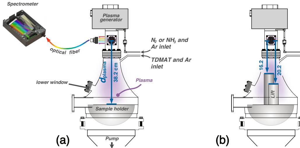
FIG. 2. Schematic drawings of the shower-head reactor (Fiji 200) and its main constituting components. (a) The sample is located at its regular position d_{\text{plasma}} = 38.2 \text{ cm} and OES monitoring is shown near the plasma generator. (b) The sample position is lifted to shorten the plasma generator-to-sample distance: d_{\text{plasma}} = 16.2 or 20.2 \text{ cm} .
