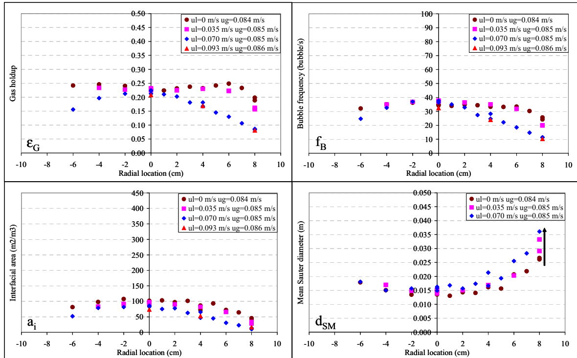
Figure 20. Local profiles at h=0.25 m for the large hole sparger ( d_0=0.001 m)
