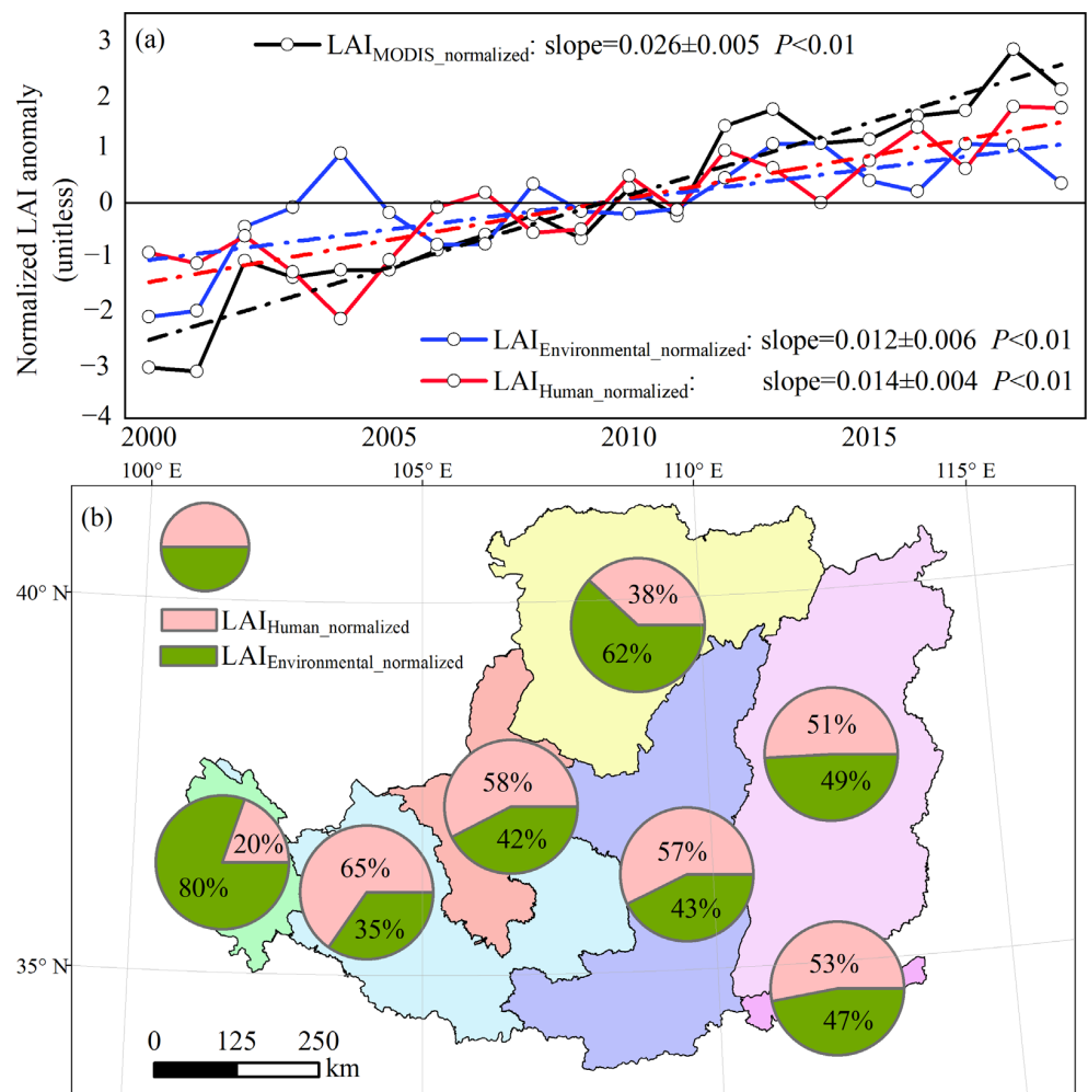
Figure 5. The influences of natural and anthropogenic factors on vegetation change in the Loess Plateau during 2000–2019. (a) The relative interannual trends of actual LAI ( \text{LAI}_{\text{MODIS\_normalized}} ), environmental change-induced LAI ( \text{LAI}_{\text{Environmental\_normalized}} ) and human land-use management-induced LAI ( \text{LAI}_{\text{Human\_normalized}} ). Anomalies were calculated as the difference between the normalized LAI for a given year and the average value during the study period. (b) The relative contribution of environmental change and human land-use management to the actual LAI trends for each province.
