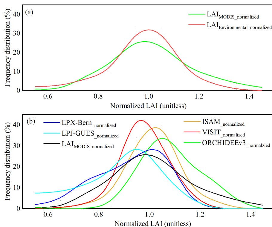
Figure 10. The frequency distribution of normalized LAI. (a) The frequency distribution of LAI MODIS_normalized and LAI Environmental_normalized ; (b) the frequency distribution of normalized MODIS LAI and normalized simulated LAI from models.
