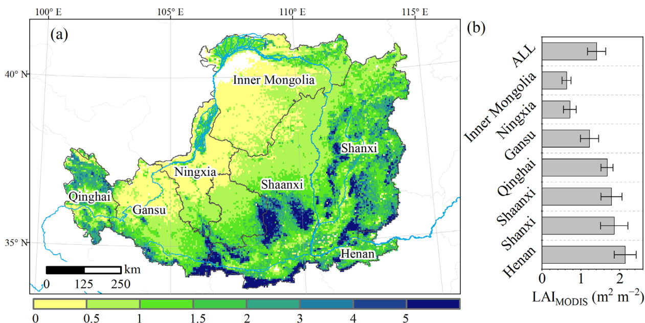
Figure 2. (a) The spatial pattern and (b) average values for each province of MODIS LAI on the Loess Plateau.
