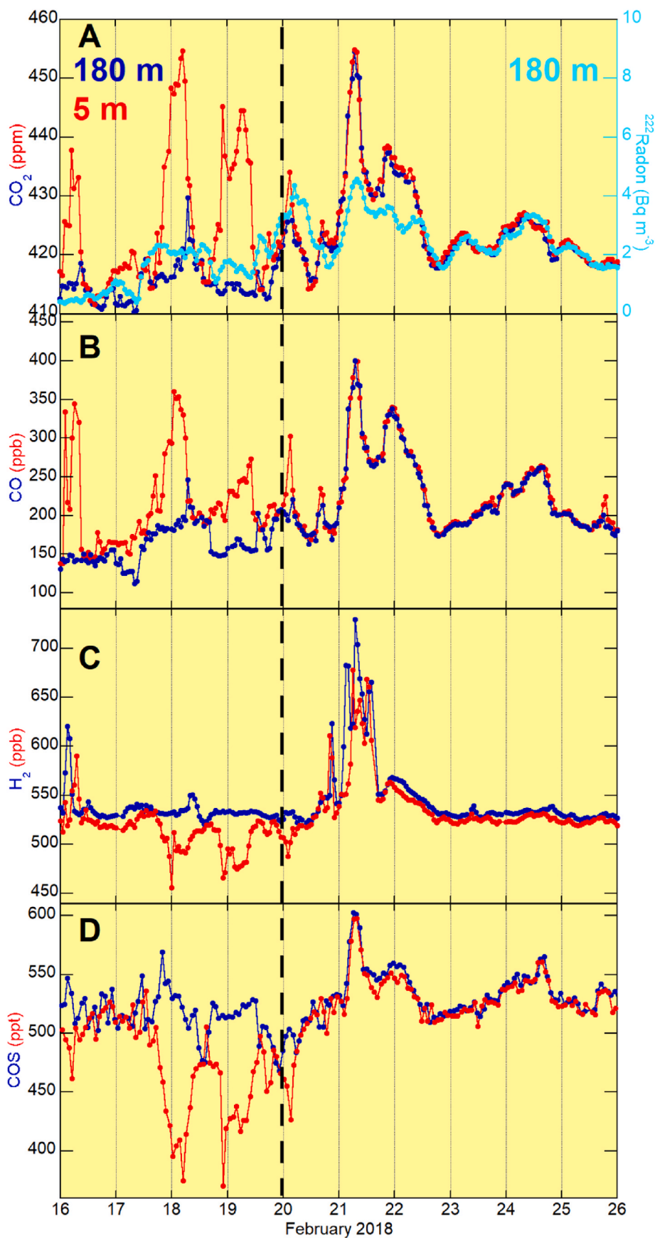
Fig. 4. ^{222}\text{Rn} activity and \text{CO}_2 mixing ratio (A), CO, \text{H}_2 and COS mixing ratios (panels B–D) during February 2018 at TRN. Sampling heights are displayed in panel A. The transition from nocturnal stratification to vertical mixing is depicted as a vertical bold dashed line.
