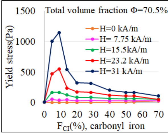
Fig 14a Bingham yield stress versus solid volume fraction of CI particles. Total volume fraction: \Phi=70.5\% .
