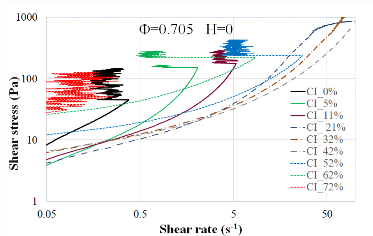
Fig.4 Total volume fraction \Phi=0.705 for different volume percentage F_{CI} of carbonyl iron. Raw curves in plate-plate geometry. The dotted lines are for fractions F_{CI} \geq 50\% ; the dashed dotted lines are for fractions F_{CI} which do not present a DST transition.
