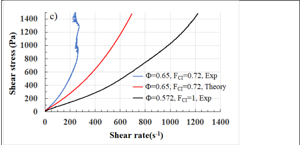
Fig.11 Comparison between experiment(blue line) and homogenization theory(red line) for a) F_{CI}=0.91 ; b) F_{CI}=0.815 , c) F_{CI}=0.72 The solid black line corresponds to the experiment for pure iron at the respective interstitial volume fraction volume fraction \Phi'_{CI}=0.628 , \Phi'_{CI}=0.602 , \Phi'_{CI}=0.572
