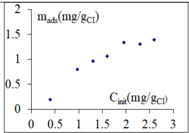
Fig. B2 -Adsorption isotherm of PPP44 on carbonyl iron particles in water at T=20°C
