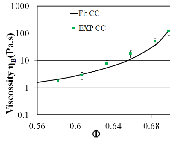
Fig.8a Bingham viscosity of a suspension of pure CC particles versus the volume fraction. The solid line is a fit by Eq. (3)
