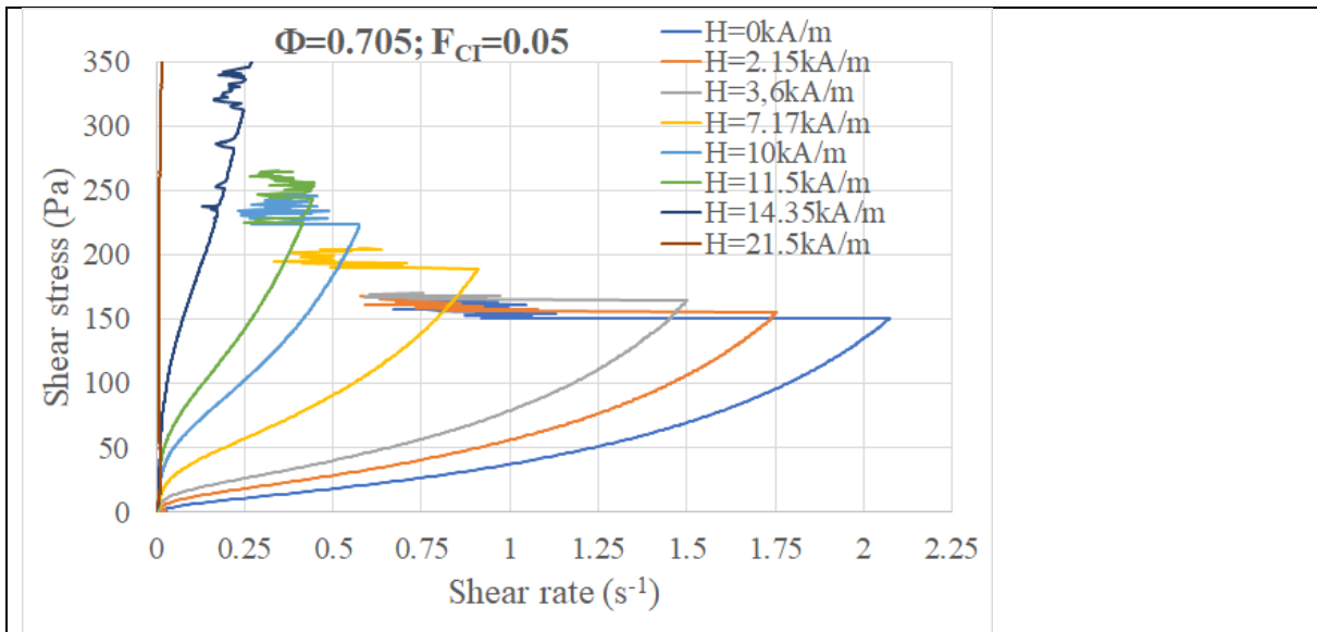
Fig. 15 Evolution of the rheology with the magnetic field for a solid volume fraction of magnetic particles: F_{CI}=5\% and a total volume fraction of solid \Phi=0.705
