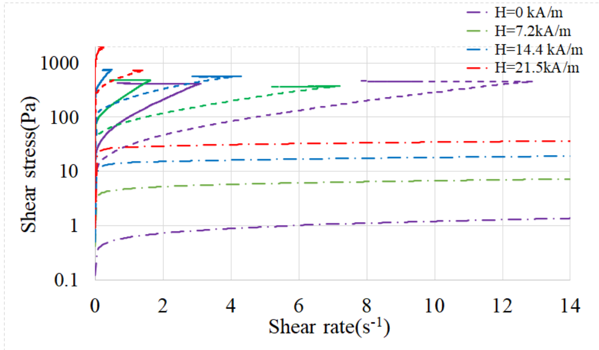
Fig.12 Stress versus shear rate for three series of identical magnetic fields H=0 kA/m, 7.2 kA/m, 14.4 kA/m, 21.5 kA/m. Dashed dotted lines: pure CI suspension at \Phi=0.23 . Dashed lines bidisperse suspensions: \Phi=0.73 ; F_{CI}=0.32 . Solid lines \Phi=0.74 , F_{CI}=0.31 . In the three suspensions \Phi_{CI}=V_{CI}/V_{tot}=0.23
