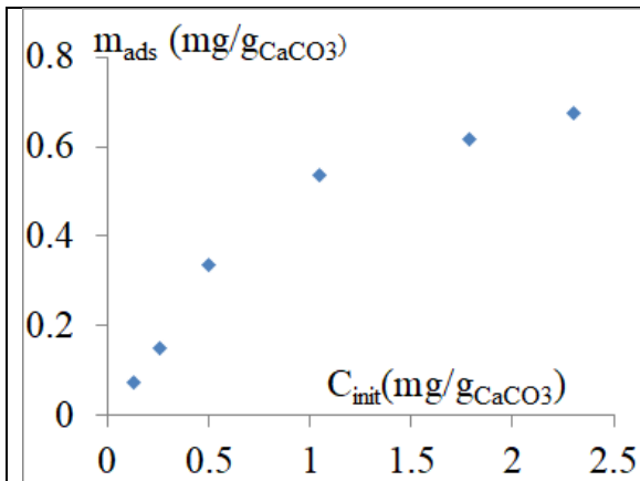
Fig. B1 -Adsorption isotherm of PPP44 on CaCO 3 particles in water at T=20°C
