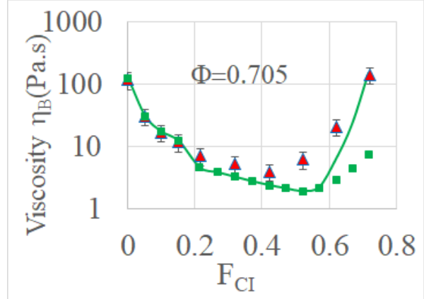
Fig.9b Bingham Viscosity of a mixture CaCO 3 /CI particles versus the solid volume fraction of CI particles. Red triangles: experiment; Green squares: Eq. (7). Green line: with a shell of volume fraction Φ s =0.563
