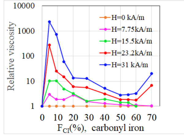
Fig 14b Relative viscosity \eta_B(H)/\eta_B(H=0) versus solid volume fraction of CI particles. Total volume fraction \Phi=70.5\%
