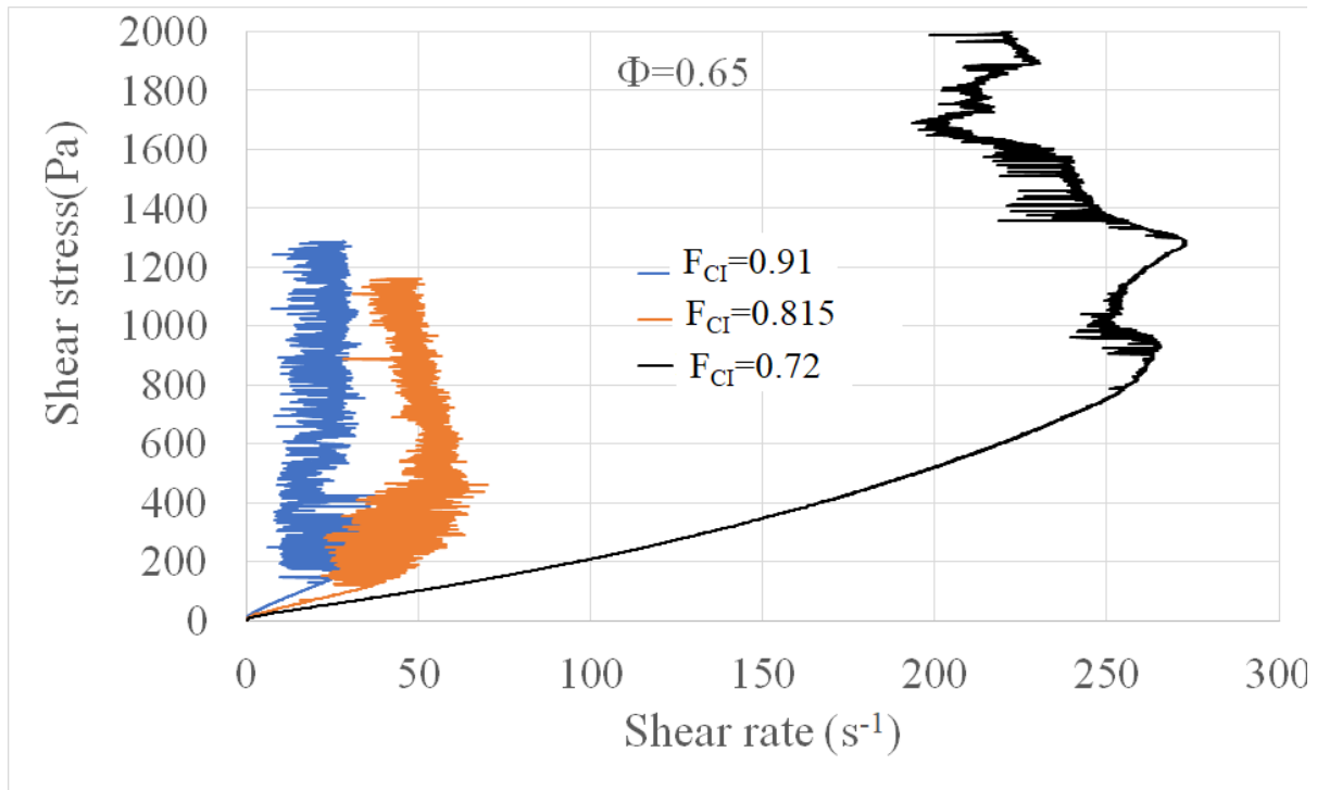
Fig10 Shear stress versus shear rate in cylindrical Couette geometry; total volume fraction: \Phi=0.65 and CI volume percentage of solid: F_{CI}=0.91 ; F_{CI}=0.815 ; F_{CI}=0.72 .
