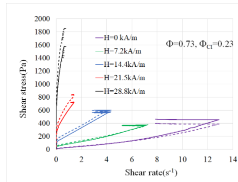
Fig.13b Same as Fig.12 in linear scale for \Phi=0.73 , \Phi_{CI}=0.23 . The dashed lines are the raw curves and the solid lines the corrected curves using Eq (2).
