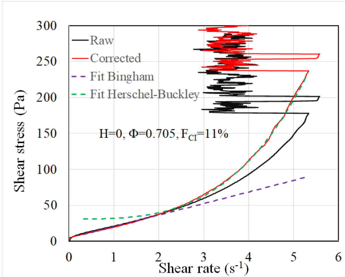
Fig.5 The black curve is the raw one for F_{CI}=0.11 . The solid red line is the corrected one given by Eq. (2). The green dashed line is the fit of the corrected curve with the Herschel Buckley law and the purple dashed line with the Bingham law.
