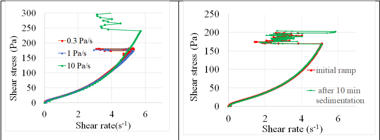
Fig. 3a Effect of the rate of rising stress for the three rates: 0.3, 1, 10 Pa/s. Total volume fraction: \Phi=0.705 ; solid fraction of \text{CaCO}_3 : F_{CC}=89\%
