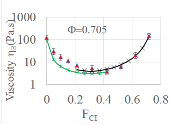
Fig.9a Bingham Viscosity of a mixture CaCO 3 /CI particles versus the solid volume fraction of CI particles. Red triangles: experiment; Green line and black line from the maximum volume fraction of a mixture of bidisperse spheres obtained from simulation (Farr et al. 2009)
