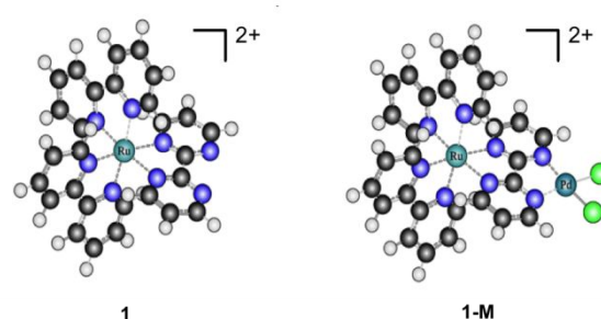
Figure 1. Structure of 1 [\text{Ru}(\text{bpy})_2(\text{bpym})]^{2+} ( \text{bpy} = 2,2'-bipyridine; \text{bpym} = 2,2'-bipyrimidine) (left) and 1-M ( \text{M} = \text{Pd} ) for [\text{Ru}(\text{bpy})_2(\text{bpym})]^{2+} coordinated to \text{PdCl}_2 (right).
