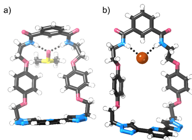
Fig. 5 Views of the solid state structure of (a) 8 and (b) 8-Br - . Dichloromethane solvate in the structure of 8 and all solvents and the TBA cations in the structure of 8-Br - are omitted for clarity. Note, that the structure of 8-Br - has Z' = 2 , only the lower-numbered macrocycle and anion are shown.
