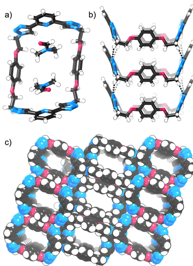
Fig. 4 Views of the solid state structure of 3 : (a) view of a single macrocycle and DMF solvates; (b) view showing inter-macrocycle C–H...N hydrogen bonds; (c) spacefilling view of nanotube structure.
