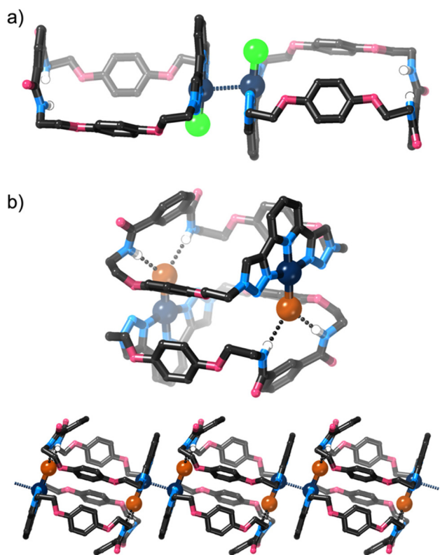
Fig. 8 X-ray crystal structures of (a) [\text{Pd}\cdot\mathbf{8}\cdot\text{Cl}]\text{BF}_4 and (b) [\text{Pd}\cdot\mathbf{8}\cdot\text{Br}]\text{BF}_4 . Solvent molecules and most hydrogen atoms omitted for clarity. The structure of [\text{Pd}\cdot\mathbf{8}\cdot\text{I}]\text{BF}_4 is very similar to that of [\text{Pd}\cdot\mathbf{8}\cdot\text{Cl}]\text{BF}_4 but does not feature a short Pd...Pd contact (Fig. S50†).
