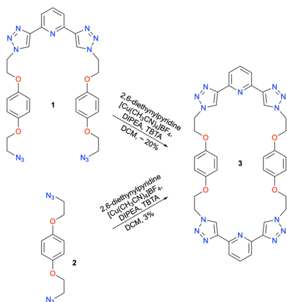
Scheme 3 Low yielding but facile syntheses of 3 .
