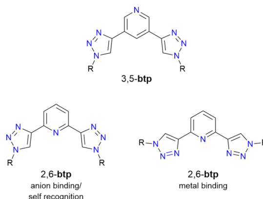
Fig. 1 Structures of two isomers of btp including both common conformations of the 2,6 isomer. The 3,5 isomer is often functionalised through either N -alkylation of the pyridine ring or incorporation of halogen groups at the 5-position of the triazole ring for anion recognition applications.
