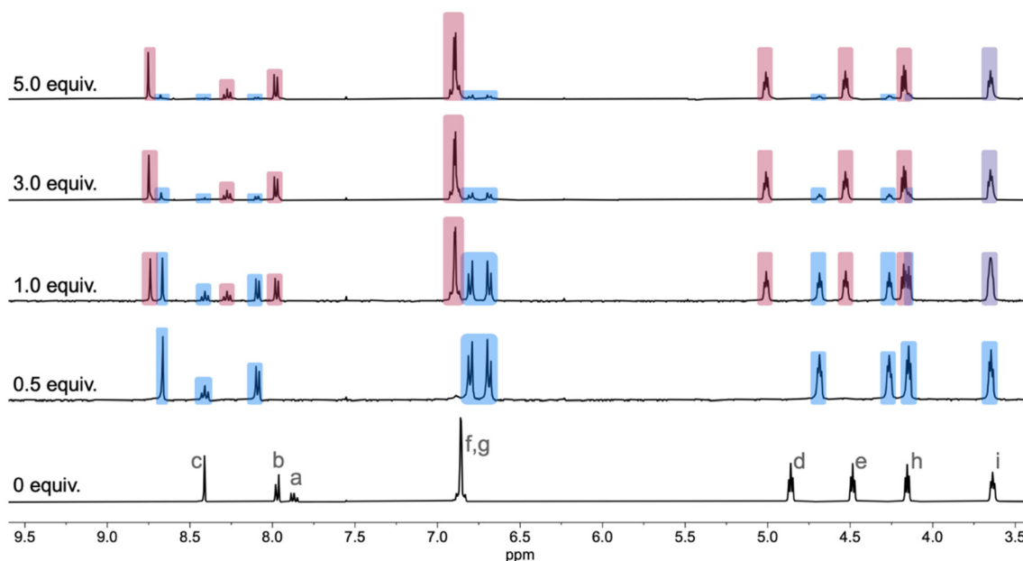
Fig. 3 Partial ^1\text{H} NMR spectra of diazide 1 upon addition of [\text{Zn}(\text{OH}_2)_6](\text{ClO}_4)_2 . Peak labelling corresponds to atom labelling shown in Scheme 1. Peaks assigned to the \text{ML}_2 species are coloured blue, peaks assigned to the \text{ML} species are coloured maroon. An expanded version of this figure including additional equivalents of \text{Zn}^{2+} is provided as Fig. S22† (2.0 mM 1 in \text{CD}_3\text{CN} , 400 MHz, 298 K).
