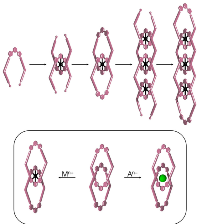
Fig. 2 Planned synthesis of btp -containing catenanes using a sequence of metalation and CuAAC reactions to generate new btp motifs. The inset shows the potential of a resulting catenane to bind metals through bis-terdentate coordination, or anions through C–H...anion hydrogen bonds.
