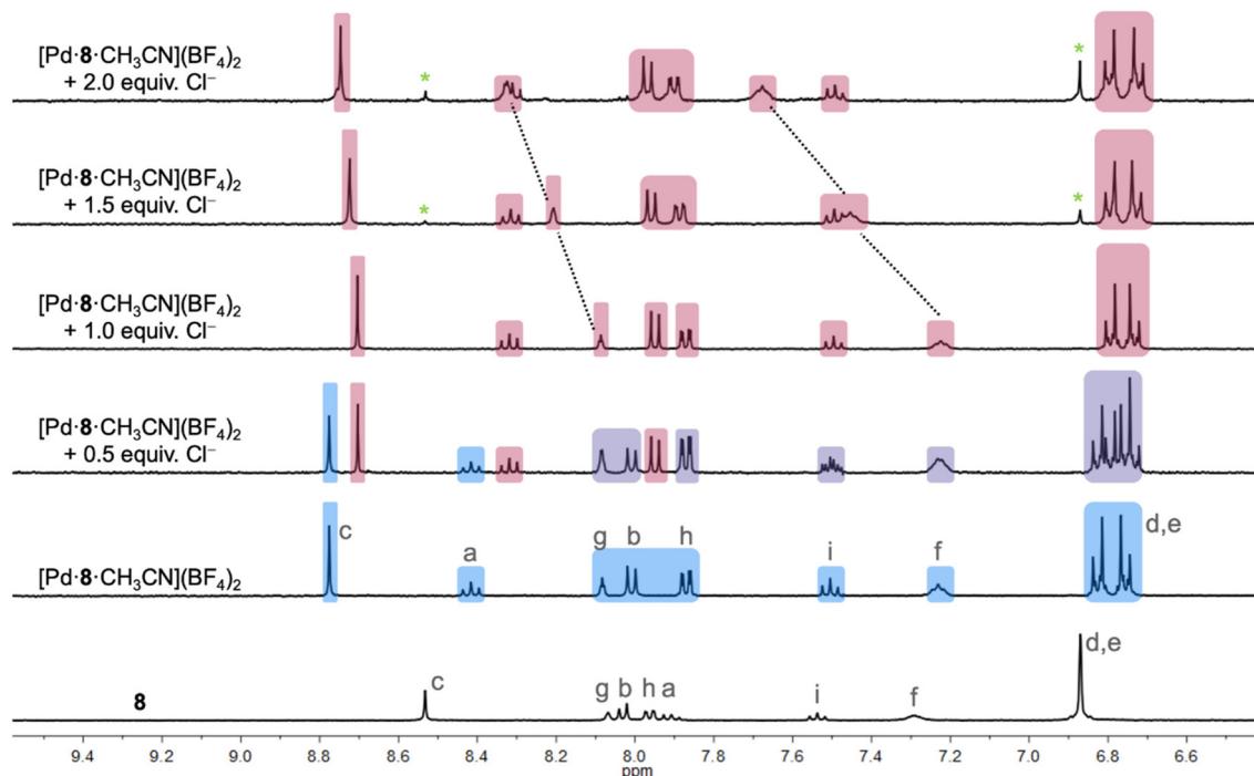
Fig. 7 Partial ^1\text{H} NMR spectra of 8 , and [\text{Pd}\cdot\text{8}\cdot\text{CH}_3\text{CN}]\text{BF}_4 upon addition of TBA-Cl. Peak labelling corresponds to atom labelling shown in Scheme 4. Peaks corresponding to [\text{Pd}\cdot\text{8}\cdot\text{CH}_3\text{CN}](\text{BF}_4)_2 are coloured blue, peaks corresponding to [\text{Pd}\cdot\text{8}\cdot\text{Cl}]\text{BF}_4 are coloured maroon, and peaks corresponding to both are coloured purple. Peaks corresponding to the re-formation of uncomplexed 8 are indicated with green asterisks. An expanded version of this figure including additional equivalents of \text{Cl}^- and a wider spectral window is provided as Fig. S41 † (1.0 mM in \text{CD}_3\text{CN} , 298 K, 400 MHz).
