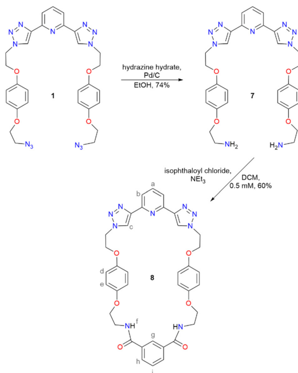
Scheme 4 Synthesis of btp diamide macrocycle 8 .
