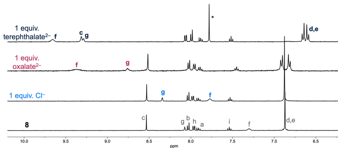
Fig. 6 Partial ^1\text{H} NMR spectrum of 8 upon addition of TBA·Cl, TBA 2 ·oxalate or TBA 2 ·terephthalate (1.0 mM 8 in \text{CD}_3\text{CN} , 298 K, 400 MHz). Peaks that show significant movement on anion addition are labelled corresponding to atom labelling shown in Scheme 4; * indicates the peak arising from terephthalate anion.
