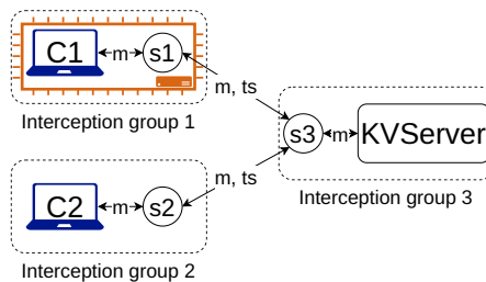
(b) Adding causally consistent communication (cc) layer to our key-value store: with two client ( c1 , c2 ), one KVServer ( kv ) and three CC-sidecars ( s1 , s2 , s3 ). m denotes a message and ts denotes a vector clock.
