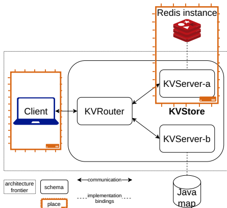
(a) A key-value store (S-KV) composed of two shards and a router.
